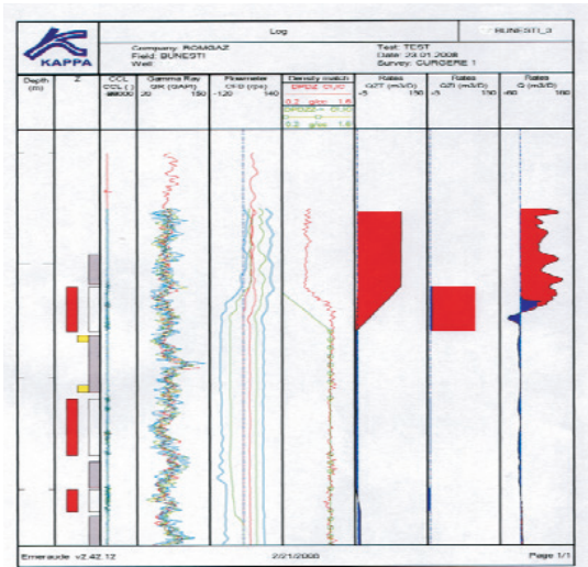
Fig. 5. PLT log interpretation – Well X Bunesti
