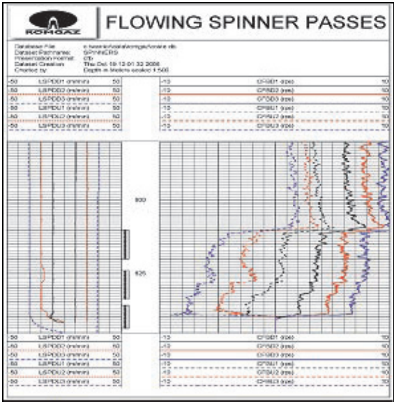
Fig. 4. PLT log – Spinner passes – Well X Rusi
