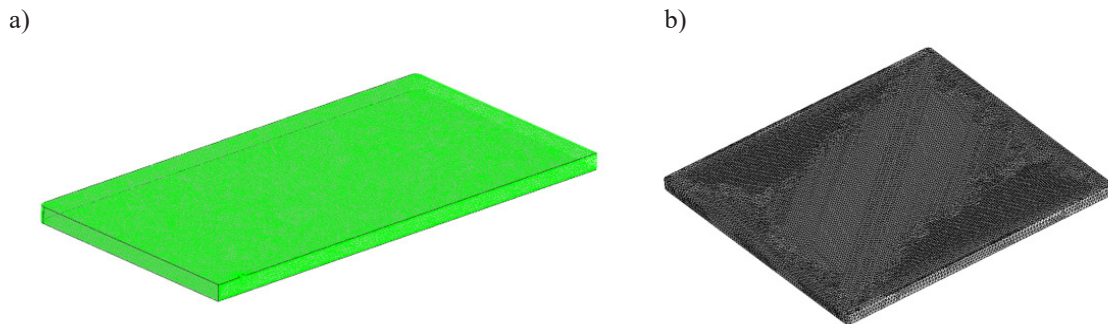
Fig. 8. Meshes in ANSYS CFX (a) and Cadmould 3D-F (b)
