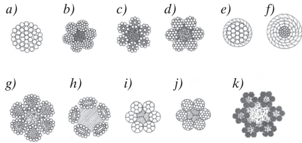
Fig. 2. Selected sections of the lifting ropes [12]: a) single thread; b) double thread; c) double thread; d) Warrington double thread; e) closed structure with one armour of wires; f) closed structure with two armours of z-wire and trapezoidal wires; g) double strand with triangular strands; h) double strand with strands; i, j) double strand with seamless strands; k) triple strands with round strands
