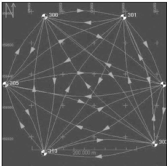
Fig. 8. Baseline calibration
