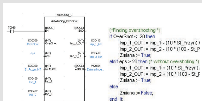
Fig. 2. Example of Function Block FB with Structure Text ST
