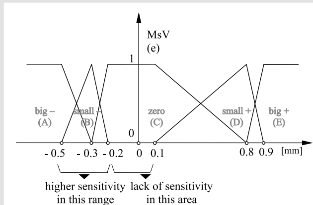
Fig. 4. Error membership functions (second input)
