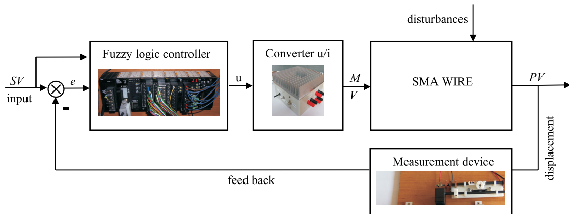
Fig. 1. Block diagram control system for a prototype of linear position actuator (Kwaśniewski 2008)
