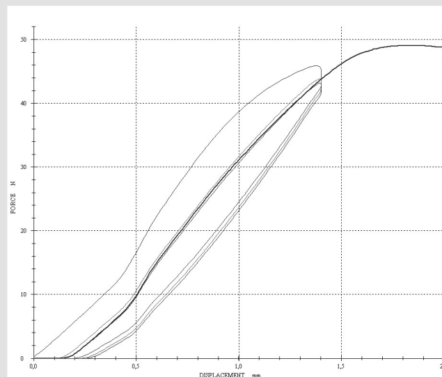
Fig. 4. Cyclic distortion and destruction of PBT GF10 sample after H-T 2 ageing cycle
