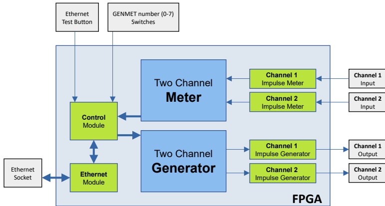
Figure 7. The GENMET architecture
