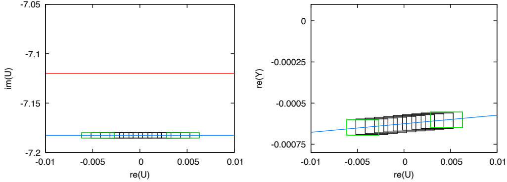
Figure 5: A closeup of the crossing of the trajectory through the section \{\text{Re } U = 0\} projected onto U on the left (compare with Figure 4), and onto coordinates (\text{Re } U, \text{Re } Y) on the right. In black we have the interval arithmetic bounds. In green, we have singled out the bounds on the trajectory for two disjoint time intervals, to demonstrate that it indeed does cross \{\text{Re } U = 0\} . In blue we have a non-rigorous plot of the trajectory, which is added to the figure as a point of reference.
