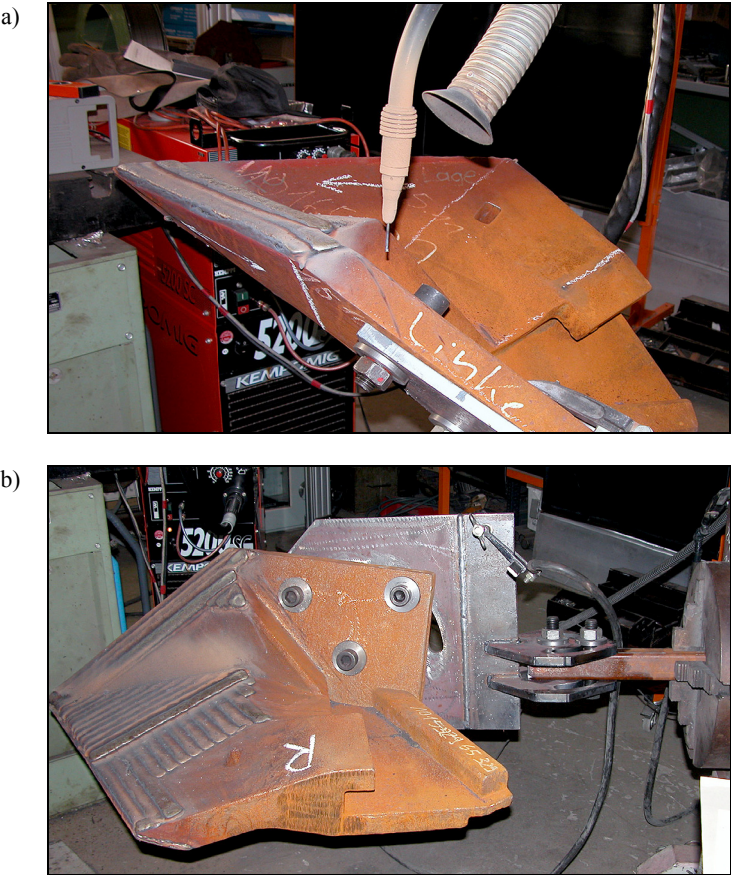
Fig. 1. Equipment and test arrangement in surfacing
