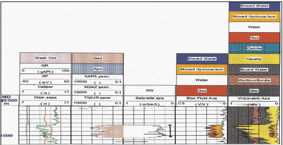
Fig. 9. Petrophysical interpretation
