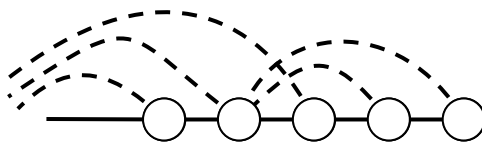
Fig. 3. Partial 1-degenerate packing of two pathlike trees, one of them having at least 4 leaves
