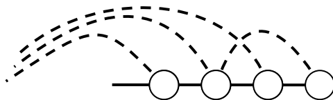
Fig. 5. Partial 1-degenerate packing in case 3(b)
