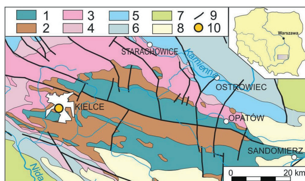
Fig. 1. Geological settings of the Świętokrzyskie (Holy Cross) Mountains with the location of the Kadzielnia Park and Underground Touristic Trail (map after Urban, Gągoł, 2008). Explanation of symbols: 1 – Cambrian, Ordovician and Silurian, 2 – Devonian, Lower Carboniferous, 3 – Permian and Lower Triassic, 4 – Middle and Upper Triassic, 5 – Lower and Middle Jurassic, 6 – Upper Jurassic, 7 – Cretaceous, 8 – Neogene, 9 – principal fault, 10 – Kadzielnia Park with Underground Touristic Trail
