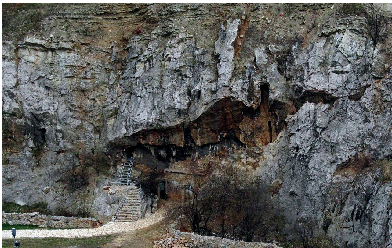
Fig. 3. The entrance to the Underground Touristic Trail in the Kadzielnia Park in 2012. Above the entrance the fault surface with characteristic contour of karst conduits is visible; in the uppermost part of the quarry face the Famennian limestone-marl-clay thin-bedded series is visible, photo J. Urban
