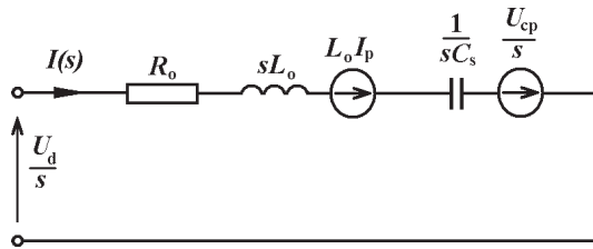
Fig. 3. Equivalent circuit of the inverter in operational form
