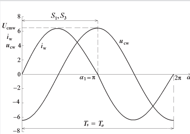
Fig. 5. Waveforms of load current i_w and voltage u_{cw} across capacitor C_s in mode II for \frac{\alpha_o}{\omega_o} = 0.1
