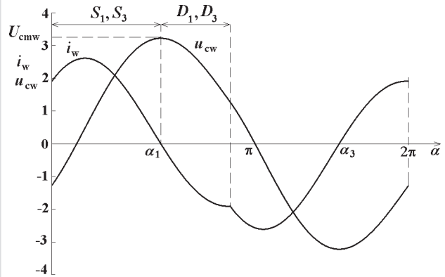
Fig. 6. Waveforms of load current i_w and voltage u_{cw} across capacitor C_s in mode III for \frac{\alpha_o}{\omega_o} = 0.1 and \frac{\omega_s}{\omega_o} = 0.83
