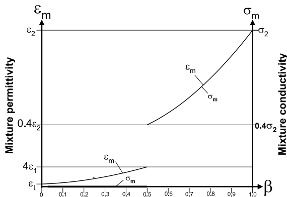
Fig. 1. Mixture permittivity and conductivity versus the volume fraction of component 2 of a homogeneous mixture of component 1 and 2. Only component 2 is conductive
