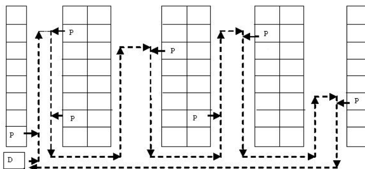
Fig. 7. Return strategy
