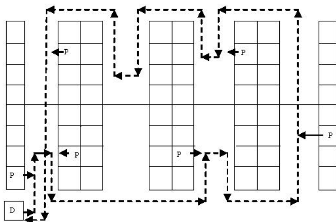
Fig. 6. Midpoint strategy
