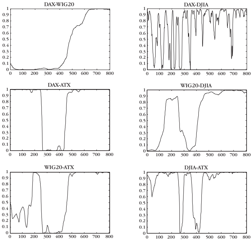
Figure 1. Smoothed probabilities (first regime)
