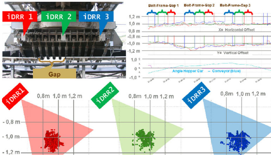
Fig. 6. Arrangement of the iDRR sensors (top left), position-time diagram of the measured values over three conveyor frames (top right) and x , y scatter diagrams over approx. 15 conveyor frames (bottom)
