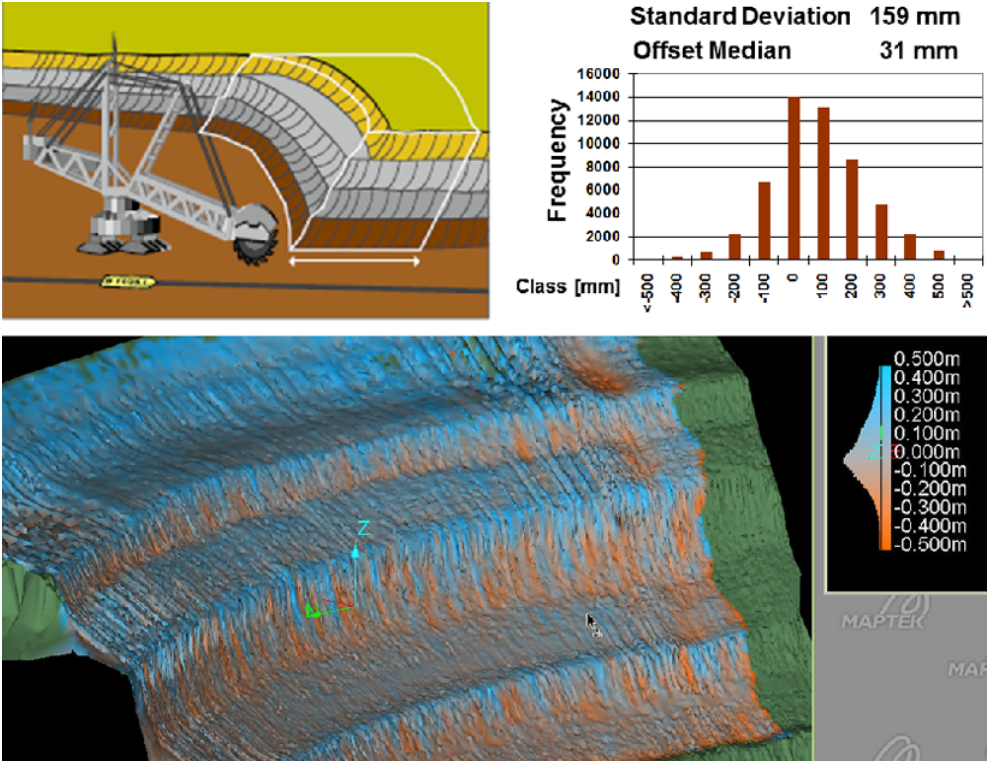
Fig. 4. ± 0,5m Color Coded Distance of the Radar Surface Measurement and the Laser Surface Measurement at good conditions (needed for the usage of the laser)
