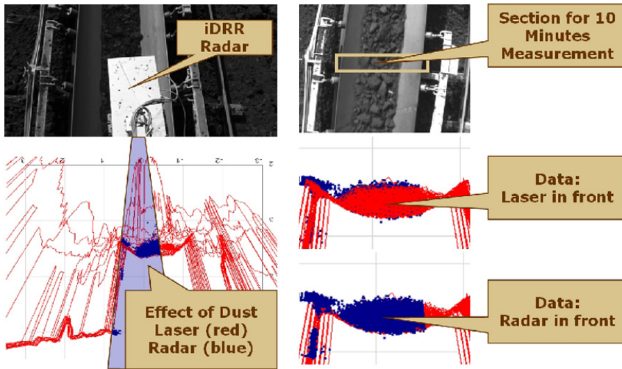
Fig. 9. Results of 2D Radar and Laser for Mass Flow Measurement
