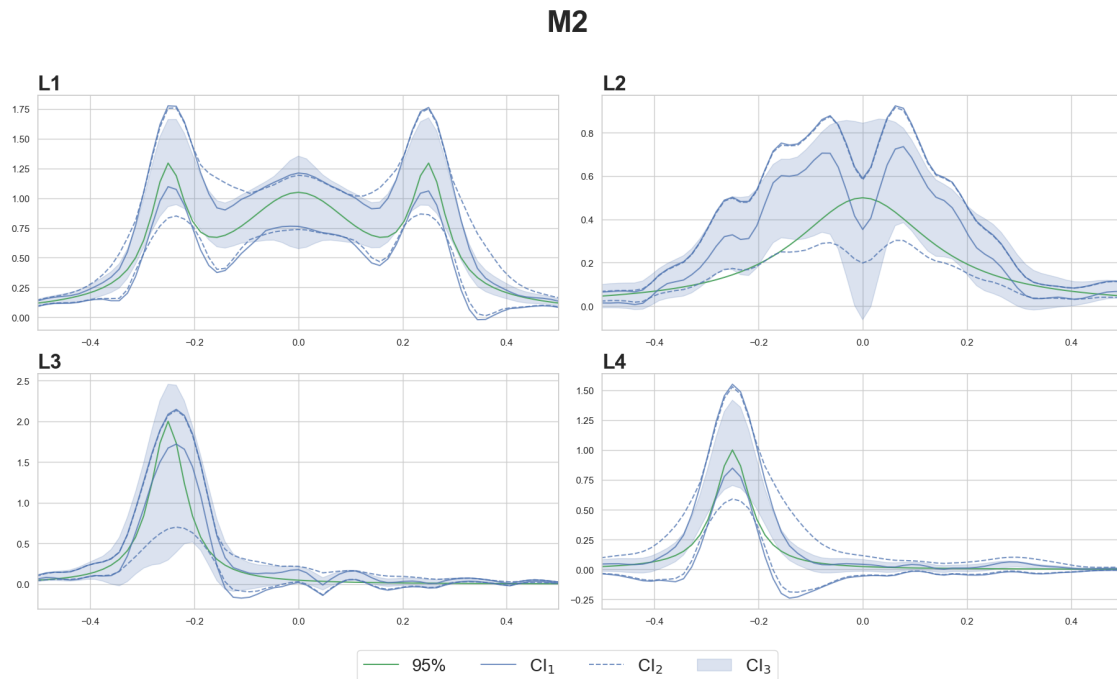
Figure 4.11: Results for M2 . Confidence intervals for the magnitude of spectral density functions for lines L1 – L4 . Green solid line: theoretical values of the magnitude of the spectral density function. Blue solid line: bounds of confidence intervals CI_1 . Blue dashed line: bounds of confidence intervals CI_2 . Blue shaded area: bounds of confidence intervals CI_3 .
