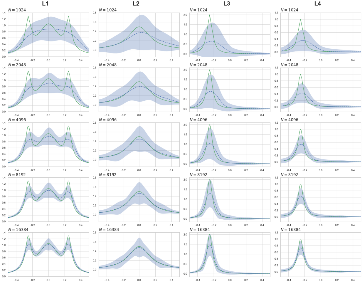
Figure 4.5: Results for M2 (the case of a known line). Green solid line: the theoretical values of the spectral density function. Blue dashed line: the estimated expectation \hat{E}(T; \omega_j^N) . Shaded blue area: the region within one standard deviation \widehat{STD}(T; \omega_j^N) . Each row represents a specific value of N . The subsequent columns (from the left) correspond respectively to lines L1 – L4 .
