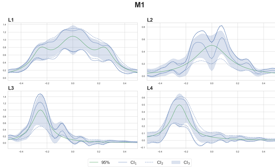
Figure 4.10: Results for M1 . Confidence intervals for the magnitude of spectral density functions for lines L1 – L4 . Green solid line: theoretical values of the magnitude of the spectral density function. Blue solid line: bounds of confidence intervals CI_1 . Blue dashed line: bounds of confidence intervals CI_2 . Blue shaded area: bounds of confidence intervals CI_3 .
