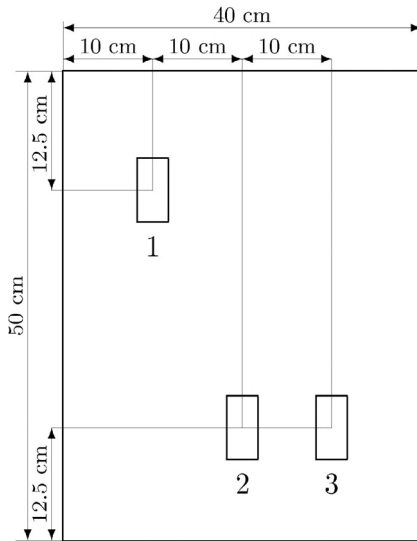
Fig. 1. Positions of MFC elements on the plate
