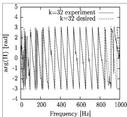
Fig. 6. Phase response of the plate with the linear equalizer
