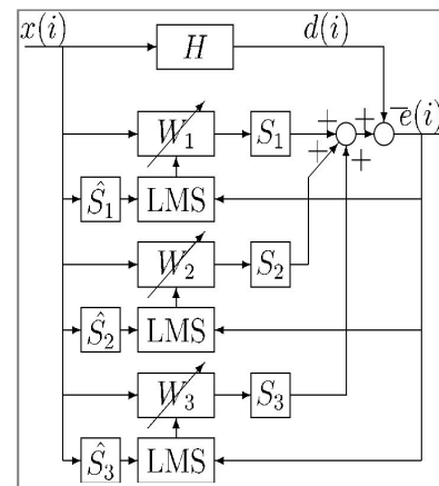
Fig. 3. Control system diagram
