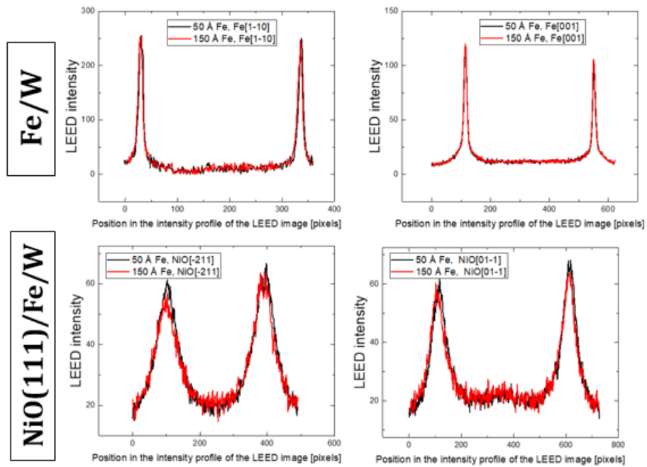
Fig.4.3 Intensity profiles as determined from corresponding diffraction patterns presented in Fig.4.2.
