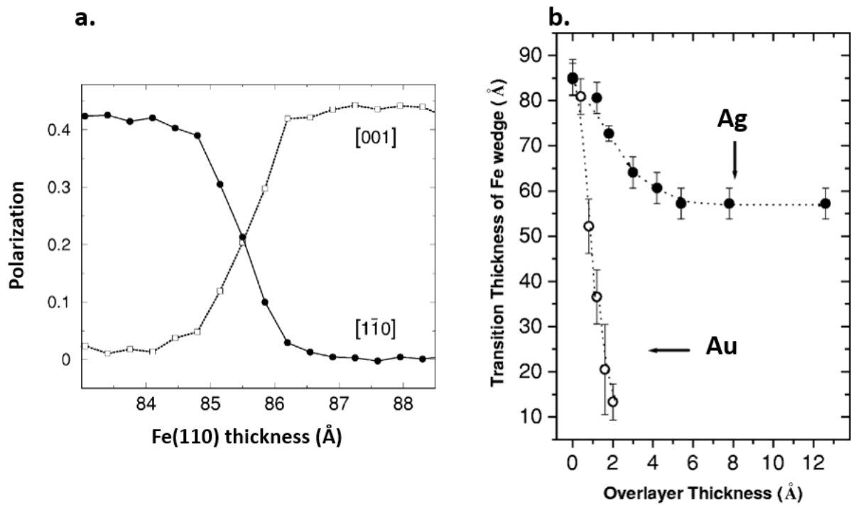
Fig. 2.4 (a) Secondary electron spin-polarization as a function of Fe(110) thickness. (b) Critical Fe thickness of SRT as a function of overlayer thickness for two studied cases, Ag and Au. These results are taken from reference. 40
