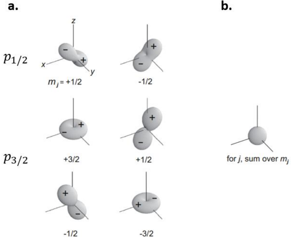
Fig. 3.8 The orbital densities corresponding to the p_j states ( p_{1/2} and p_{3/2} ) are depicted. The particular substates are denoted by quantum numbers m_j for clarity. The z -axis is chosen as the reference axis for spin quantization. Notably, the charge distributions exhibit spatial asymmetry, leading to varying X-ray absorption intensities when the E-vector aligns either parallel or perpendicular to the z -axis. The (b) figure displays the spherically symmetric charge density resulting from the summation of all m_j states, as well as the summation of m_j states within a given j . Figure adapted from reference 20 .
