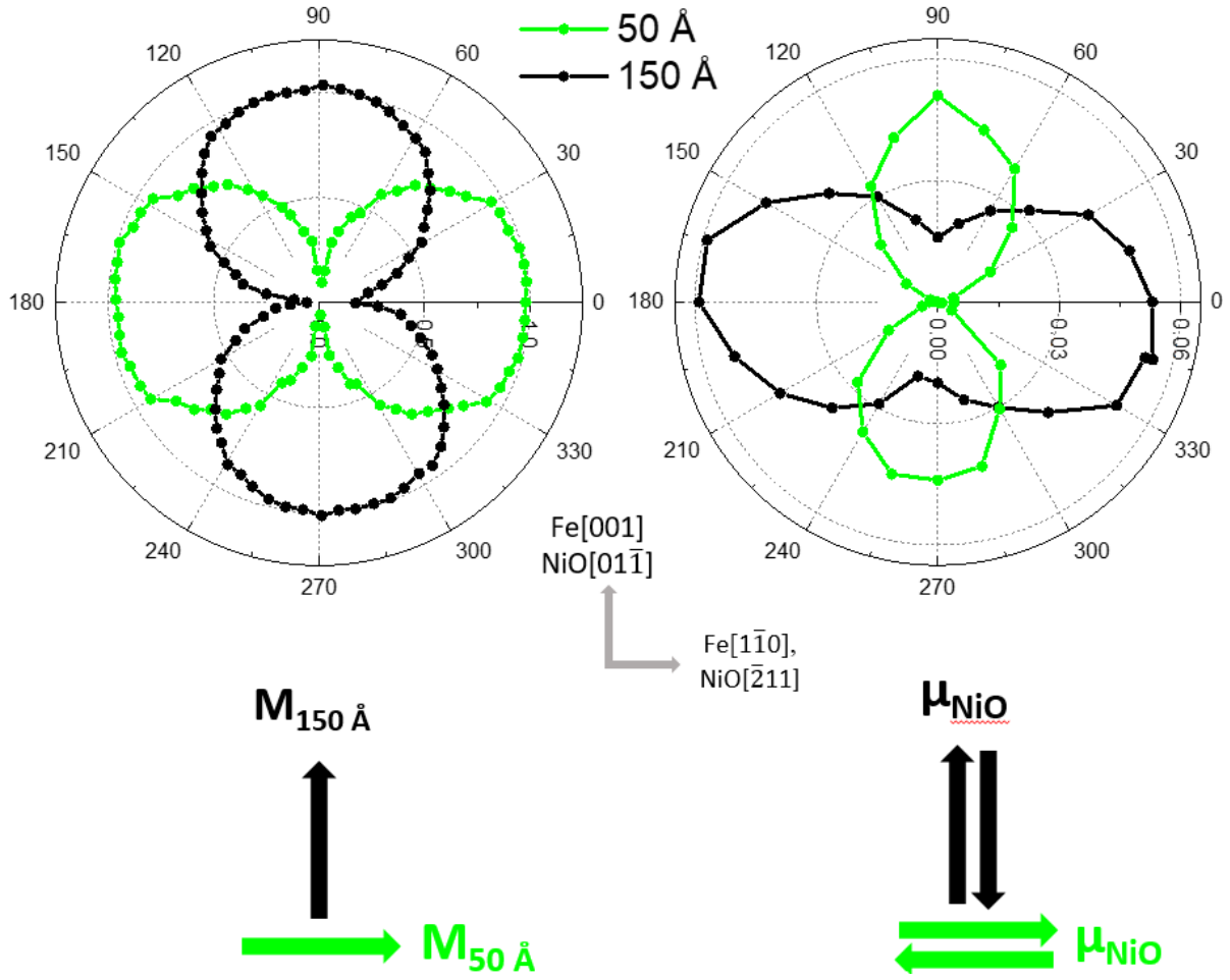
Fig 4.6 On the left side, in-plane angular dependencies of Fe magnetization in the remanent state, calculated from MOKE hysteresis loops. On the right side, XMCD magnitude defined by \Delta R_{L2} (calculated as R_{L2}(\theta = 0^\circ) - R_{L2}(\theta = 60^\circ) ) as a function of the azimuthal angle ( \varphi ). At the bottom of the image, arrows schematically indicate the easy axes of the FM Fe and AFM NiO sublayers for both sample regions. The 50- and 150-Å sample regions are coloured green and black, respectively.
