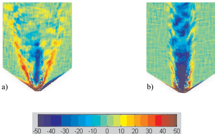
Fig. 6. Evolution of the volumetric strain \epsilon_v in sand d_{50} = 0.8 mm after 6 s of emptying rectangular silo with funnel flow: a) loose sand, smooth walls; b) dense sand, smooth walls (gravitational flow) (on the basis of the digital images)
