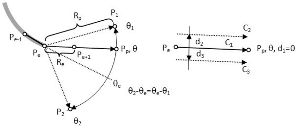
Fig. 3. The illustration of step selection rule applied in the algorithm of vein tracking:
