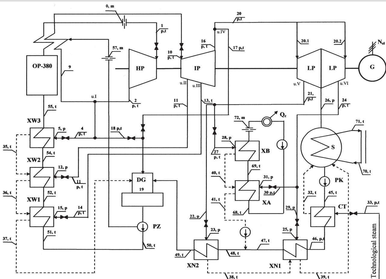
Fig. 2. Extraction condensing type unit BC-90 in the combined heat and power plant ECK S.A. – schematic flow diagram with measurement points distribution
