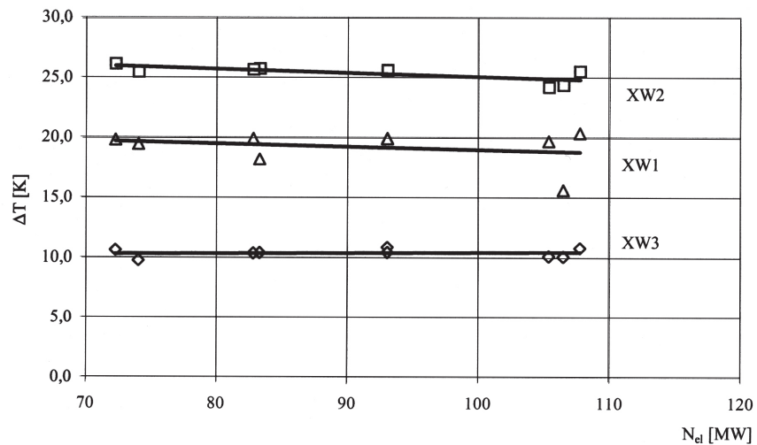
Fig. 15. Temperature difference \Delta T between the media in heaters in the range of operating loads in the heating mode of operation
