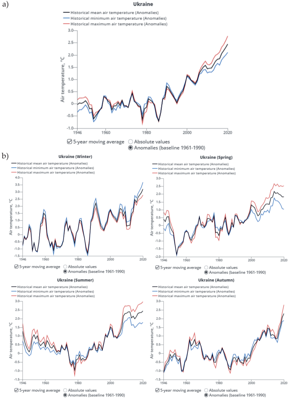
Fig. 3. Annual (a) and seasonal (b) mean, minimum, and maximum air temperatures in Ukraine for period of 1946–2020
