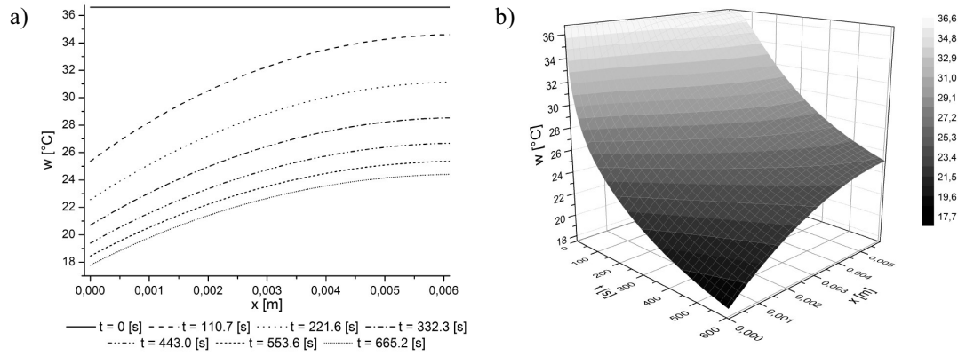
Fig. 3. Temperature distribution ^{\circ}\text{C} in case of forced convection with \alpha = 32.34 \text{ W}/(\text{m}^2 \cdot \text{K}) for a) selected values of time t [s], b) for t \in [0, 665.2] [s]
