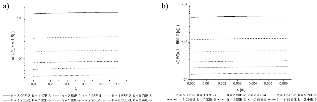
Fig. 4. Widths of the interval solutions a) U(\xi, \tau = 1.5) ; b) W(x, t = 665.2 \text{ s}) obtained with the ICN-LHS method for different values of stepsizes h and k
