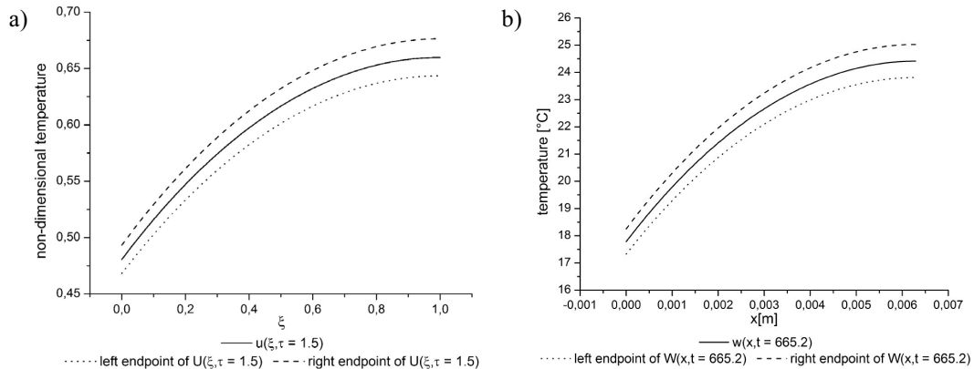
Fig. 7. The approximate and interval solutions, obtained with the CN-LHS and ICN-LHS methods for h = 1\text{E-}2 , k \approx 2.93\text{E-}5 in case of uncertainty about thermal conductivity, specific heat and mass density of dermis, given in the a) non-dimensional; b) dimensional coordinates
