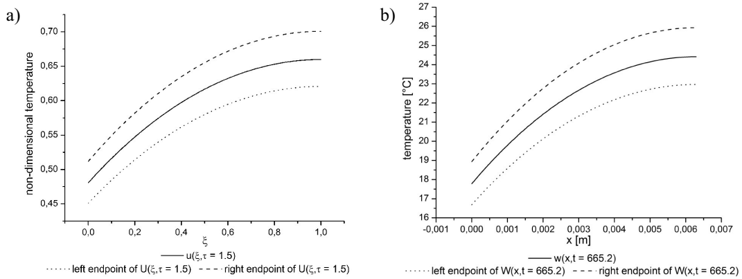
Fig. 6. The approximate and interval solutions, obtained with the CN-LHS and ICN-LHS methods for h = 1\text{E-}2 , k \approx 2.93\text{E-}5 in case of uncertainty about thickness of dermis, given in the a) non-dimensional; b) dimensional coordinates
