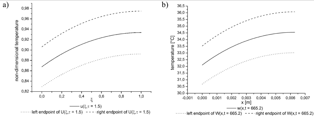
Fig. 5. The approximate and interval solutions, obtained with the CN-LHS and ICN-LHS methods for h = 1\text{E-}2 , k \approx 2.93\text{E-}5 in case of uncertainty about metabolic heat generation of dermis and subcutaneous tissue, given in the a) non-dimensional; b) dimensional coordinates
