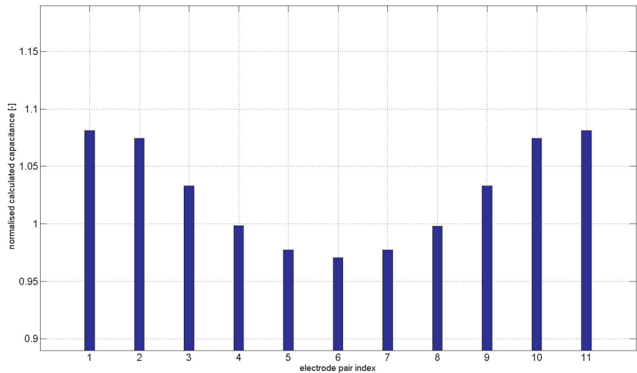
Fig. 8. Simulated normalisation data for phantom of axially symmetrical regions ( \pm 5\% concentration change): \epsilon'_I = 1.05 \cdot e_{full} , \epsilon'_{II} = 1.0 \cdot e_{full} , \epsilon'_{III} = 0.95 \cdot e_{full} from Figure 6
