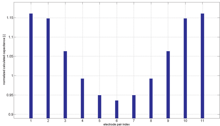
Fig. 7. Simulated normalisation data for phantom of axially symmetrical regions ( \pm 10\% concentration change): \epsilon'_I = 1.1 \cdot e_{full} , \epsilon'_{II} = 1.0 \cdot e_{full} , \epsilon'_{III} = 0.9 \cdot e_{full} from Figure 6
