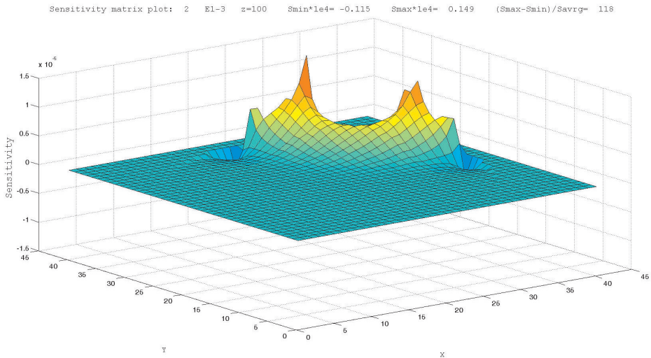
Fig. 2. Sensitivity map for C_{13}
