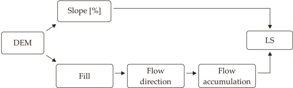
Fig. 6. Flowchart of LS factor
