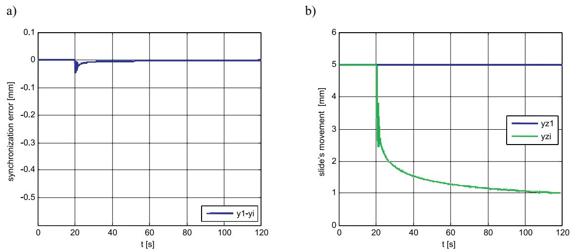
Fig. 6. Response of the system to the linear growing change of the disturbance value in the no 1 assembly: a) synchronization error; b) slide's movement in the hydraulic control valves
