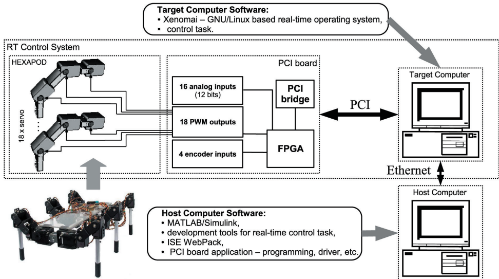
Fig. 3. The scheme of the development environment architecture
