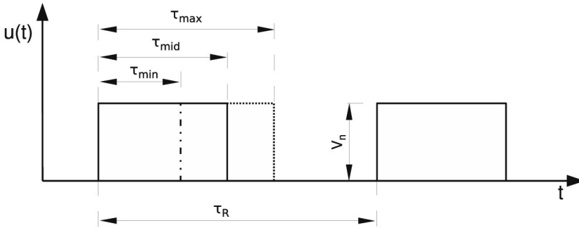
Fig. 2. The servo motor control signal: V_n = 3\text{--}4\text{ V} , \tau_{\max} = 2.1\text{ ms} is the servo motor at the right boundary position, \tau_{\text{mid}} = 1.5\text{ ms} is the servo motor at the mid-position, \tau_{\min} = 0.9\text{ ms} is the servo motor at the left boundary position, \tau_R = 20\text{ ms} is the square pulse refresh time
