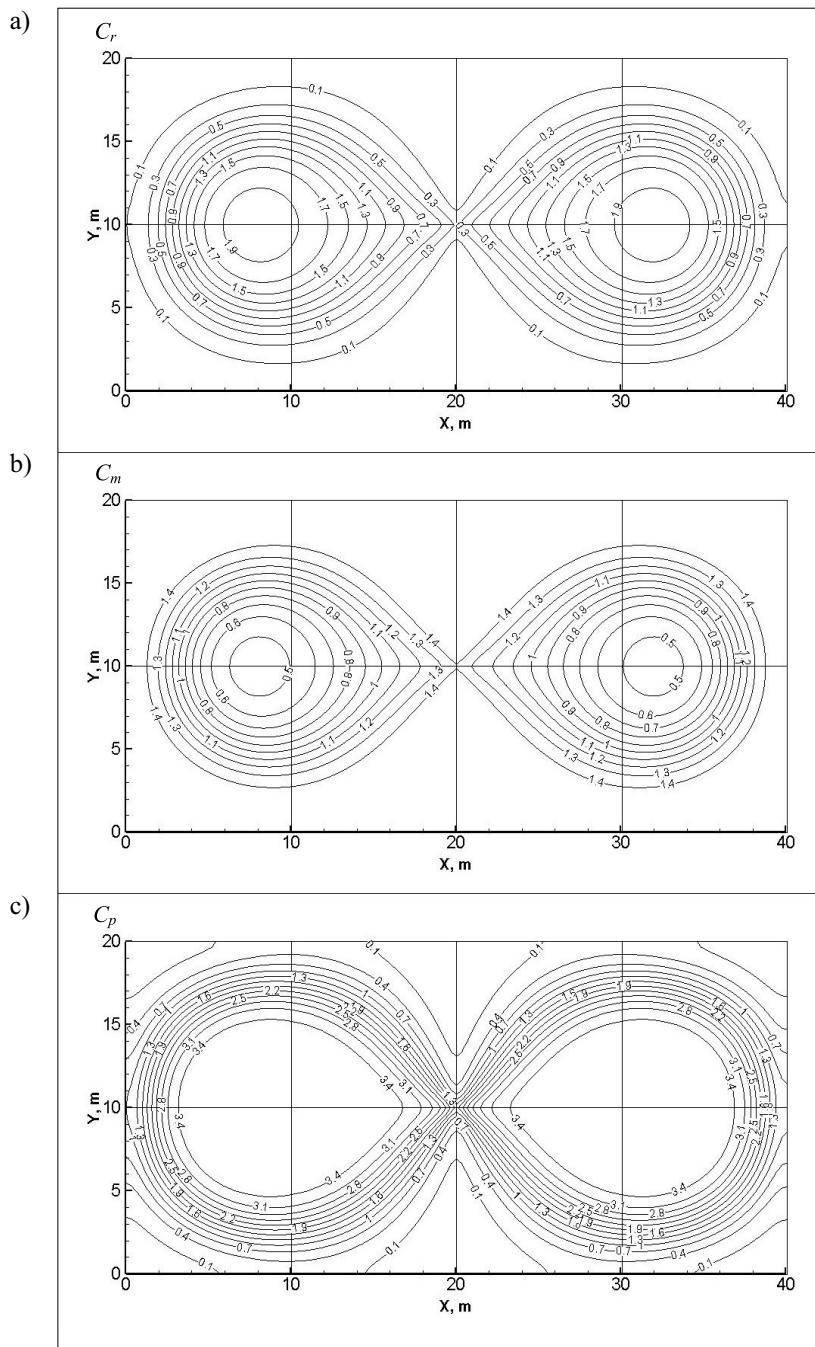
Fig. 5. Concentration isoline: a) reagent; b) useful component in solid phase; c) useful component in fluid phase, in layer at t = 100 day (horizontal section on 3 m depth)
