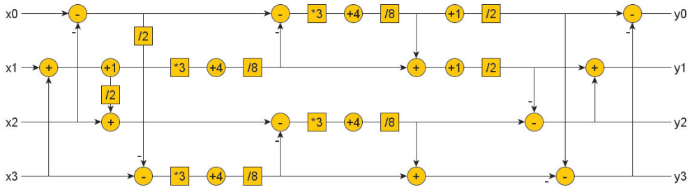
Fig. 8. Graphical diagram of data flow in Todd
