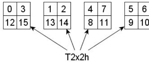
Fig. 4. Correlation between pixels in the first stage of FCT
