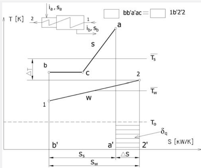
Fig. 2. Thermodynamic losses in a double-section exchanger abstracting superheated steam
