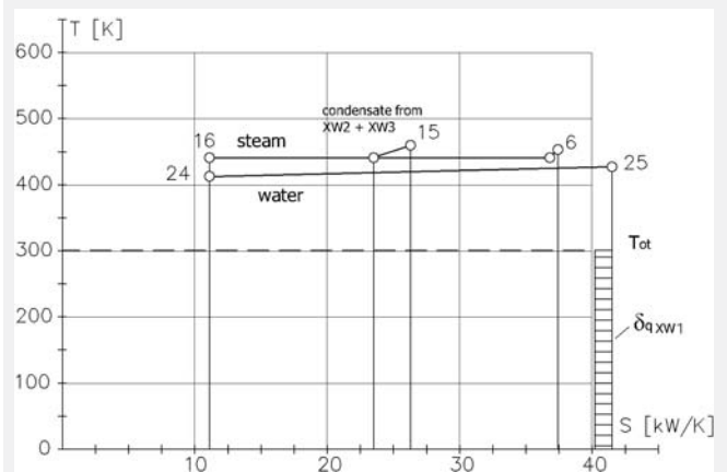
Fig. 4. Exergy loss flux \delta_{qXW1} in the heat exchanger XW1 in the heating mode of operation, for the working load N_{el} = 96.0 MW
