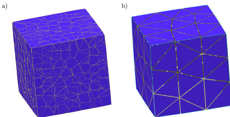
Figure 6. Result of mesh adaptation for a cube: a) initial polygonal mesh (NP=2592, NF=1778); b) after remeshing with created sizing space (NP=52, NF=100).
