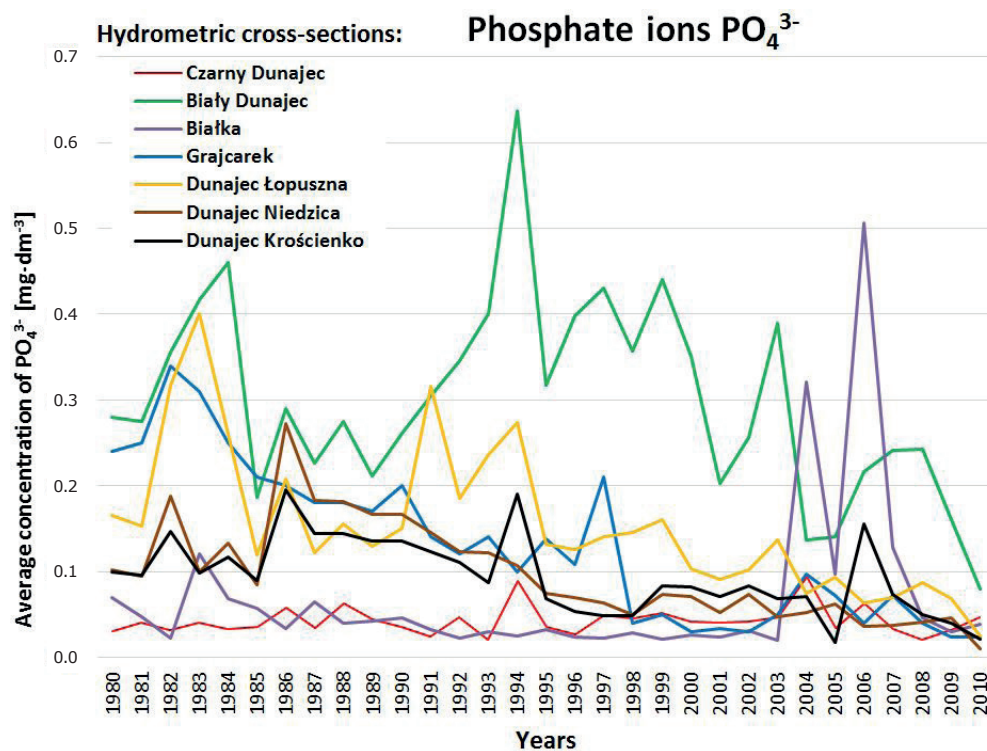
Fig. 7. Changes in average annual concentration of \text{PO}_4^{3-} [ \text{mg}\cdot\text{dm}^{-3} ] in rivers draining the upper Dunajec River basin in the years 1980–2010
