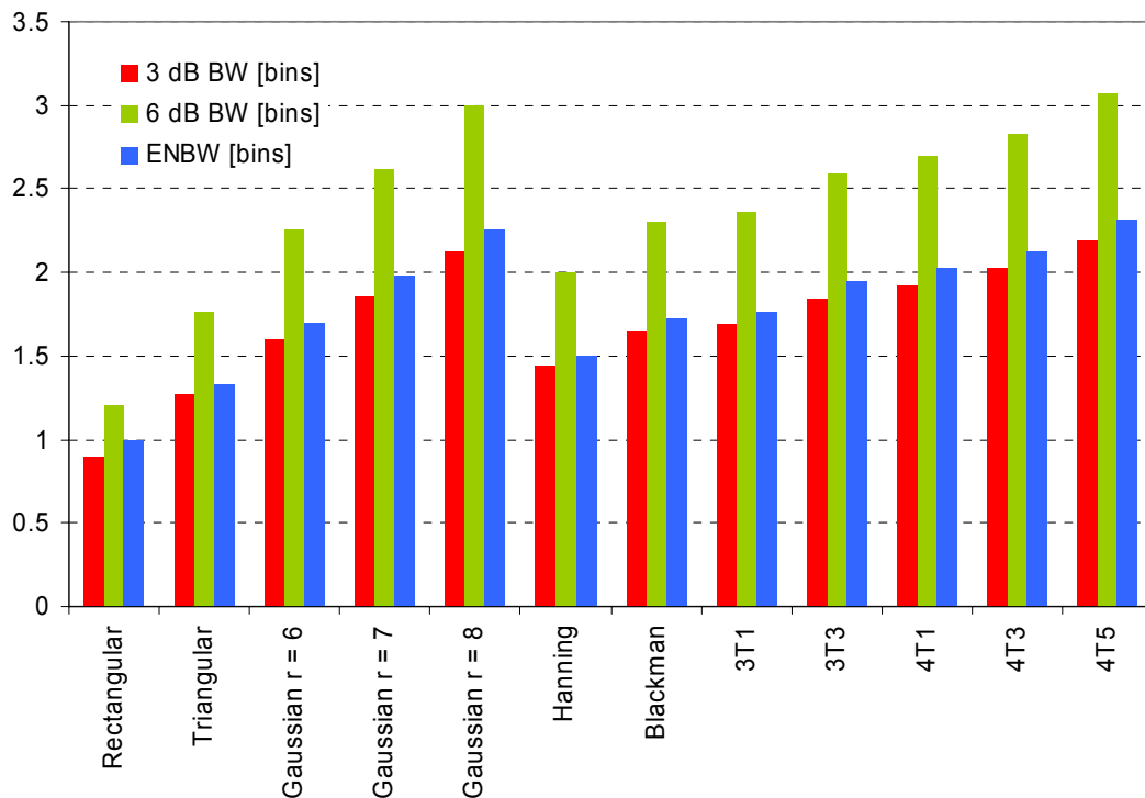
Fig. 2-7. Window properties on a bar plot. The bars are made from three columns of Table 2-1. Note that the equivalent noise bandwidth ENBW and the 3 dB main lobe width are similar for each window.
