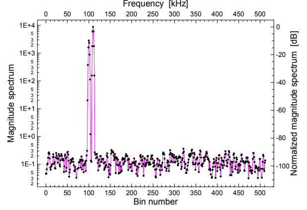
Fig. 1-5. The magnitude spectrum of the windowed samples of Fig. 1-4. The smaller spectral peak corresponds to the input component and the second to the background. With windowing, the shapes of both components are similar and they are not biased by the spectral leakage. It is seen the noise floor, previously completely drowned out by the leakage. The right vertical dB axis has the same scale as Fig. 1-3 with the spectrum of non-windowed data.
