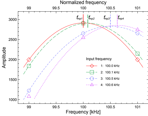
Fig. 1-7. Parabolic interpolation (1-12) for f_{in1}=100.0 kHz, f_{in2}=100.1 kHz, f_{in3}=100.5 kHz and f_{in4}=100.6 kHz. For f_{in1} lying exactly on bin 100, bins 99 and 101 have equal heights, so the corresponding interpolation result f_{mp1} is located on bin 100. When the input frequency increases, bin 99 gets smaller and 101 higher, so the abscissa of the parabola maximum shifts in the positive direction, as for f_{in2} . Bin 100 remains the largest until the input frequency is located exactly between bins 100 and 101, as for f_{in3} when they have the same heights. If the input frequency is increased further, bin 101 becomes the interpolation center as the highest one, like in the case of f_{in4} . For a decreasing input frequency the analysis is similar, resulting in symmetrical cases. Interpolation results and the corresponding errors are listed in Table 1-1.
