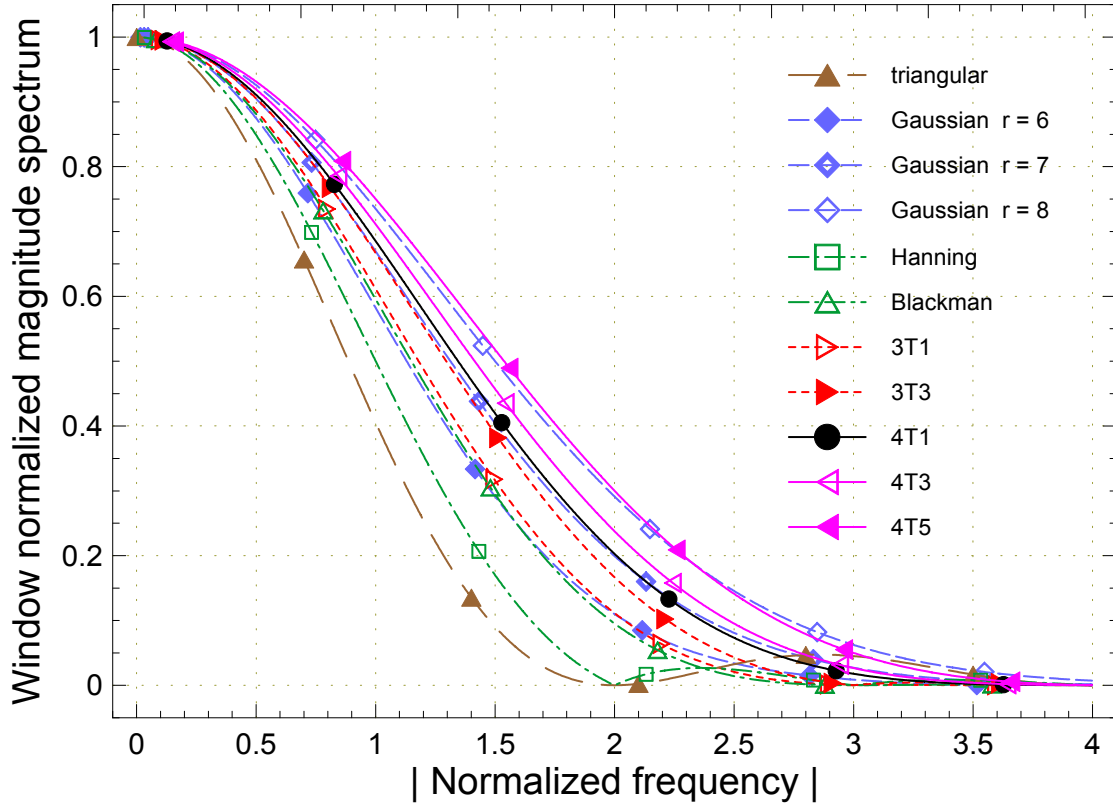
Fig. 3-3. Window magnitude spectra, shown up to |\varphi|=4 . Note that all window spectra main lobes are smooth, bell shaped curves, resembling the Gaussian shape.
