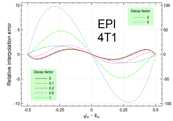
Fig. 4-33. Systematic interpolation error of the EPI method with 4T1 window for a few decay factor values. The curves for the decay factor of 0, 0.1, 0.5 and 1 are referred to the left vertical axis and the two remaining, namely 2 (green) and 5 (blue), to the right vertical axis.
