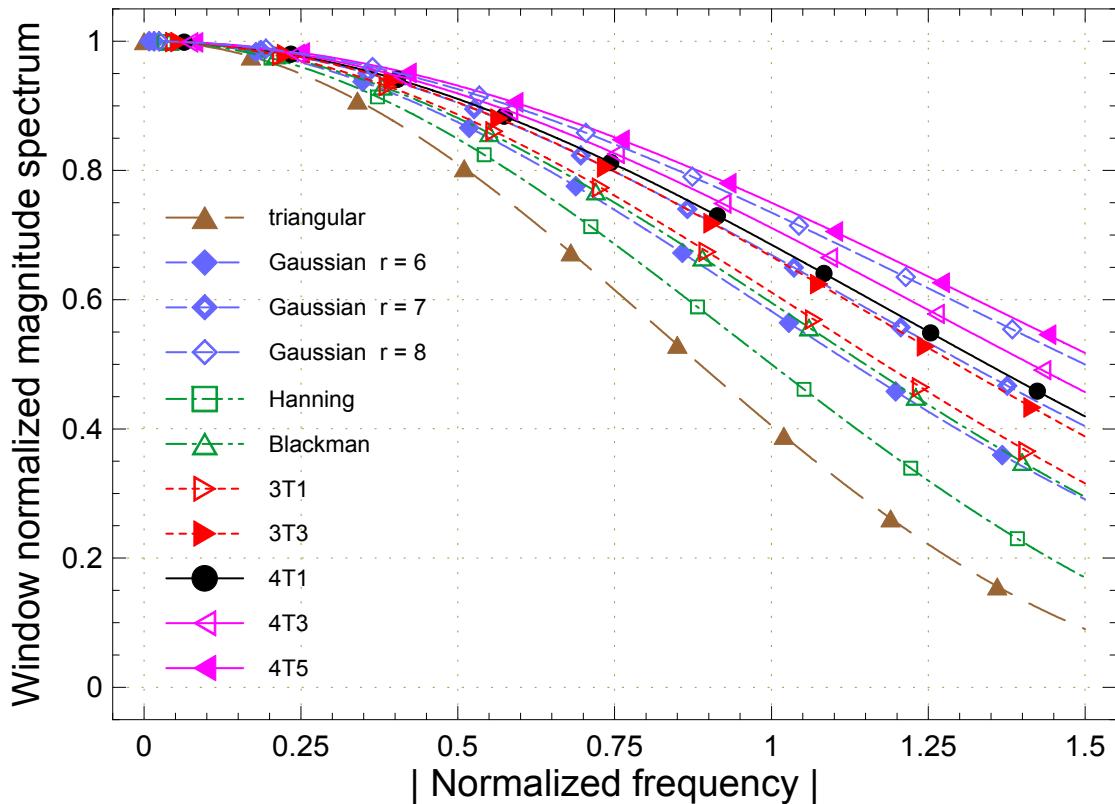
Fig. 3-1. Main lobes of window magnitude spectra, shown up to |\varphi|=1.5 , the part which is important for the interpolation methods studied in this dissertation.
