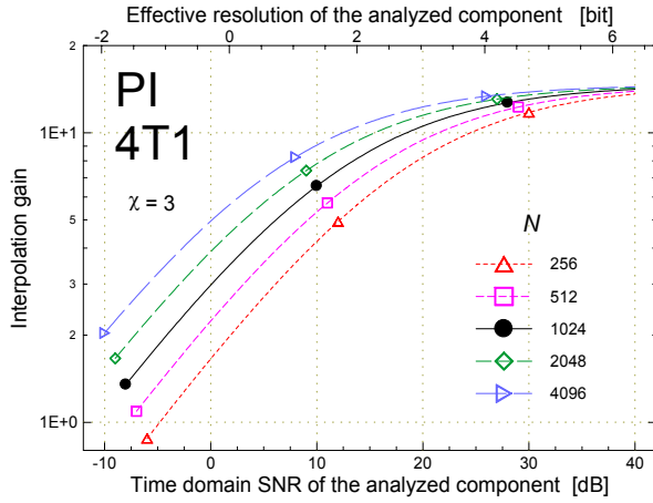
Fig. 4-13. The interpolation gain of the PI method as a function of the discrete spectrum bin number N , assuming the 4T1 windowing and the noise crest factor \chi of 3.
