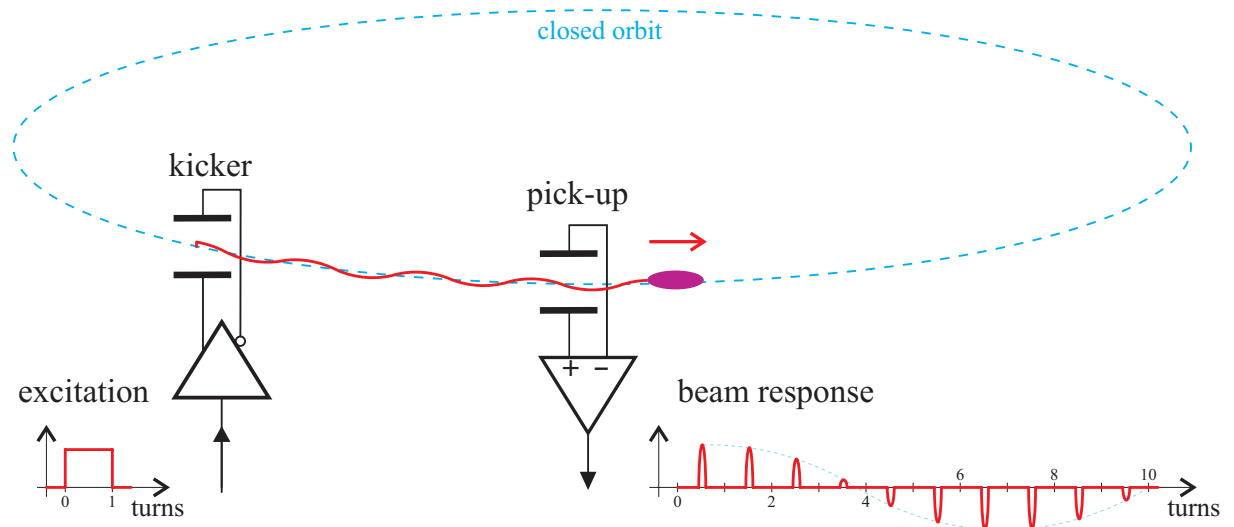
Fig. 5-2. A (simplified) block diagram of a tune measurement system for one accelerator plane. The particle beam is excited by the kicker to perform coherent betatron oscillations. The oscillations are then observed on the position pick-up. The system measures the frequency of betatron oscillations and refers it to the machine revolution frequency to yield the tune value. Due to various damping mechanisms, the oscillations last typically for a period in the order of one hundred turns.
