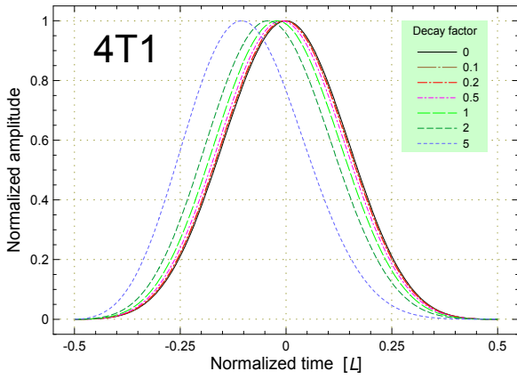
Fig. 4-30. Modified 4T1 window shapes of Fig. 4-29, but normalized to compare the window shapes. As seen, the shapes become asymmetric.
