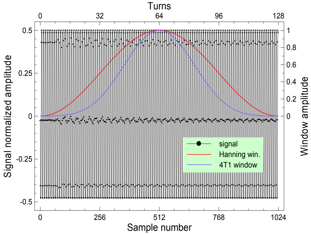
Fig. 5-7. The beam signal from the LEIR BBQ system after a small beam kick, vertical machine plane. The 12-bit samples were taken at the rate of 8 th harmonic of the revolution frequency, so there are 8 samples per machine turn. The large signal is the revolution frequency content and the betatron signal, seen as modulation of the signal zero-crossings, is much smaller. The two windows used in the example are also plotted.
