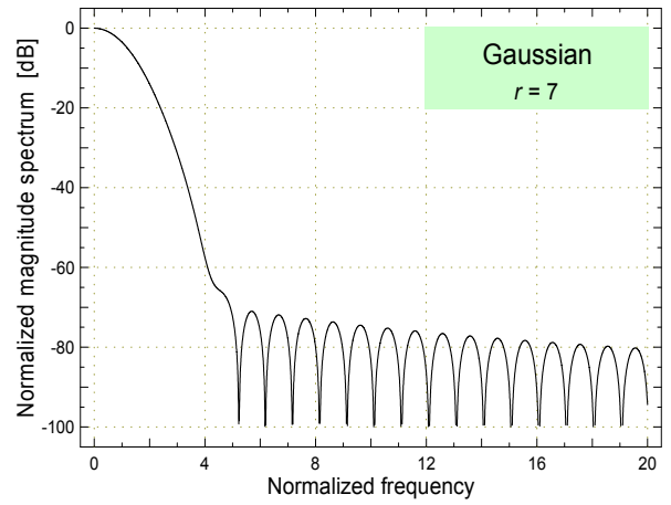
Fig. 2-11. Magnitude spectrum of the Gaussian window of length 7\sigma (i.e. truncated at \pm 3.5\sigma ).
