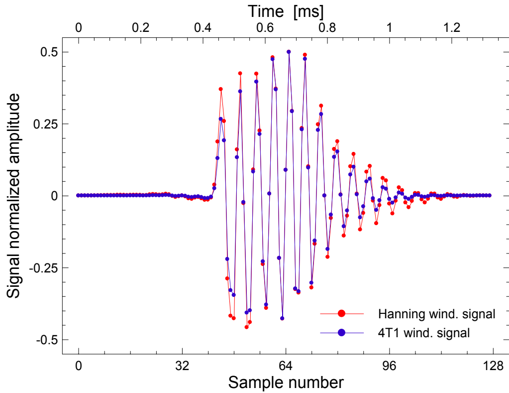
Fig. 5-4. The samples of Fig. 5-3 windowed according to the Hanning and 4T1 functions.
