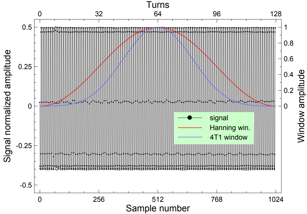
Fig. 5-16. The beam signal from the LEIR BBQ system after a small beam kick, horizontal machine plane. The 12-bit samples were taken at the rate of 8 th harmonic of the revolution frequency, so there are 8 samples per machine turn. The large signal is the revolution frequency content and the betatron signal, seen as modulation of the signal zero-crossings, is much smaller. The two windows used in the example are also plotted.
