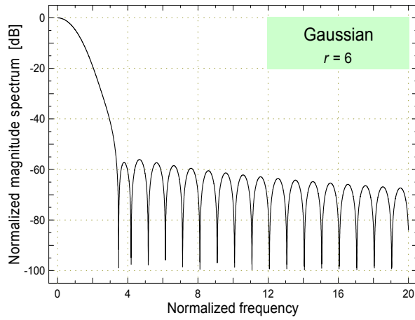
Fig. 2-10. Magnitude spectrum of the Gaussian window of length 6\sigma (i.e. truncated at \pm 3\sigma ).
