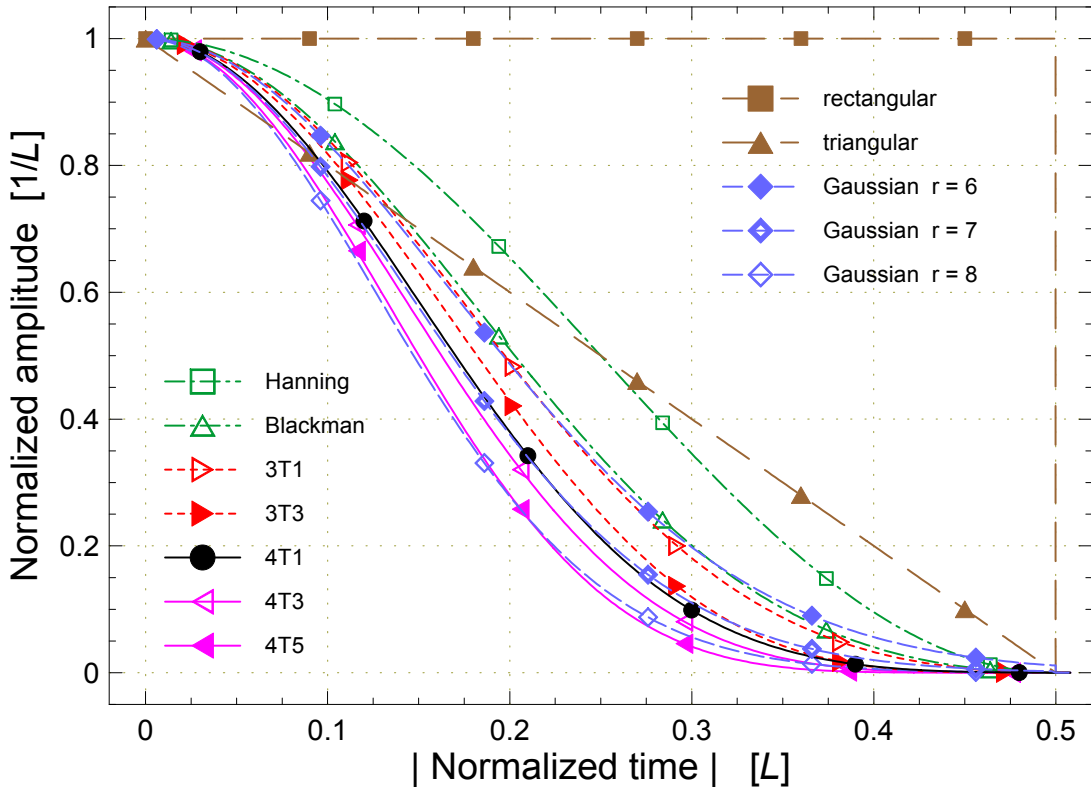
Fig. 2-5. Windows considered in this dissertation. They are symmetric, so only their halves are plotted to better reveal differences between the windows. The further paragraphs include window descriptions and the following figures – their corresponding magnitude spectra.
