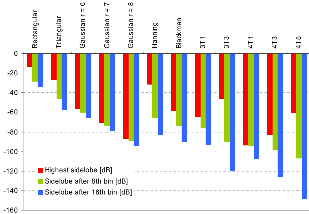
Fig. 2-6. Window spectral properties on a bar plot. The bars are made from three columns of Table 2-1. Differences between bars in each triplet describe the window sidelobe fall-off.
