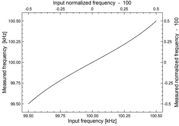
Fig. 1-8. Frequency f_{mp} from the parabolic interpolation (1-12) as a function of the input frequency f_{in} . The upper and right axes are scaled with normalized frequency \varphi . The upper axis origin is on the bin k_m = 100 being the interpolation center. The deviation from the straight line f_{mp} = f_{in} is due to interpolation errors.
