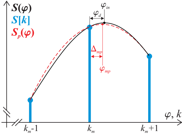
Fig. 3-1. An example of the parabolic interpolation.
