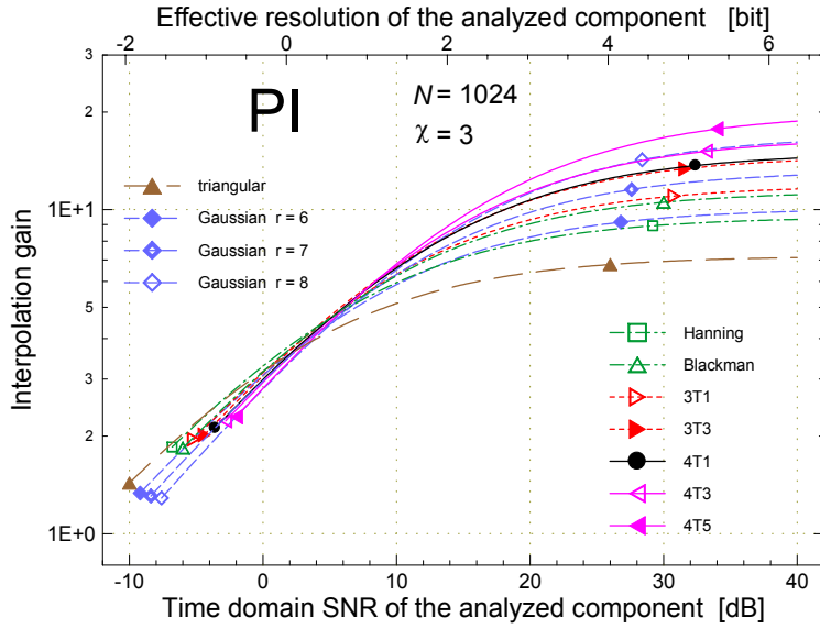
Fig. 4-9. Interpolation gain of the PI method as a function of the time domain SNR of the analyzed component for the windows considered in this dissertation, assuming 1024-point discrete spectra and the noise crest factor \chi of 3.
