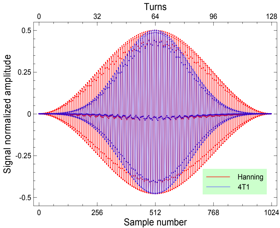
Fig. 5-8. The samples of Fig. 5-7 windowed according to the Hanning and 4T1 functions.
