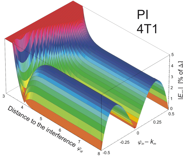
Fig. 4-19. The interpolation systematic error of the PI method with the 4T1 window as a function of the distance to the interference \varphi_{di} (of the same amplitude as the analyzed component) and the position between two spectrum bins \varphi_d = \varphi_{in} - k_{in} .
