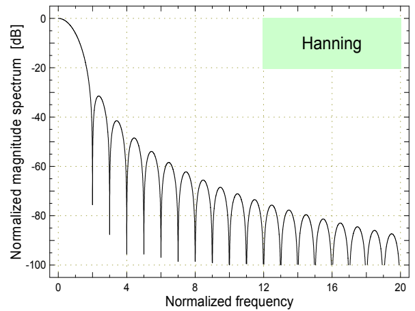
Fig. 2-13. Magnitude spectrum of the Hanning window.
