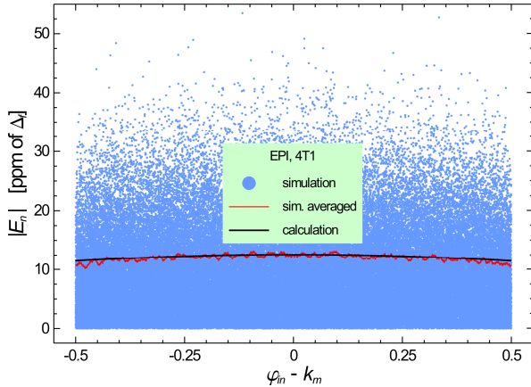
f1) EPI method, 4T1 windowing, 2048-points, effective resolution 11.0 bits. \{E_n\}_{rms} from the simulation and calculation [ppm of \Delta_f ]: 12.0 and 12.2, error -1.7 %.
