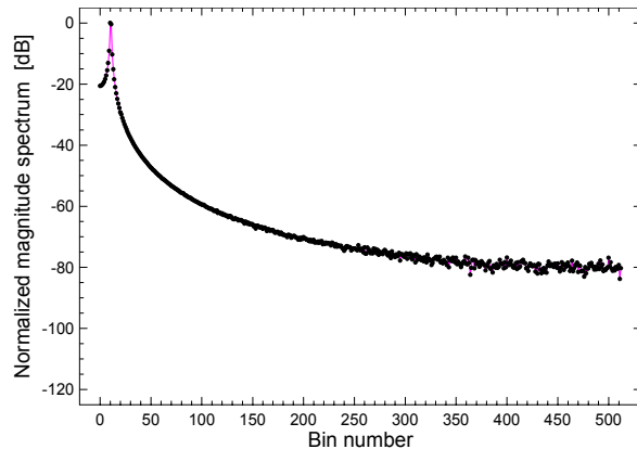
Fig. 2-2. Magnitude spectrum of the time domain sequence shown in the plot on the left. It is seen a strong spectral leakage due to the fact that the replicas of the time domain sequence do not fit on the boundaries, resulting in abrupt irregularities.
