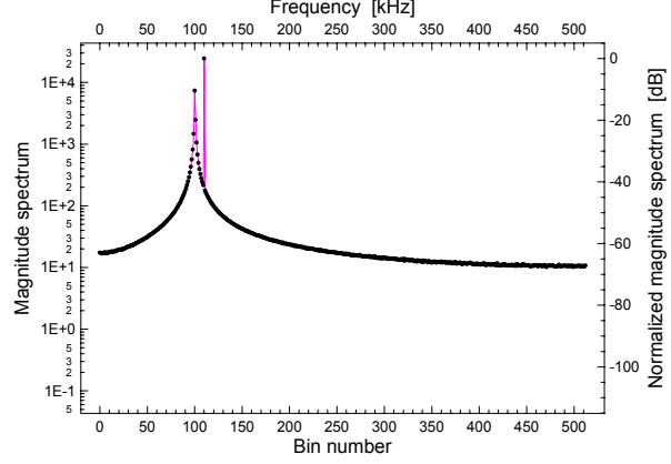
Fig. 1-3. The magnitude spectrum of N=1024 samples of the example signal shown in Fig. 1-2. The smaller spectral peak corresponds to the input component and the bigger to the background one. The input component peak is biased by the spectral leakage effect, while the background peak is narrow and biased only by the spectral leakage of the input component. The right vertical axis is scaled in dB with respect to the highest peak.
