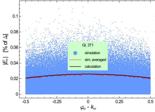
b1) GI method, 3T1 windowing, 1024-points, effective resolution 7.0 bits. \{E_n\}_{rms} from the simulation and calculation [% of \Delta_f ]: 0.0237 and 0.0241, error -1.7 %.
