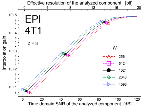
Fig. 4-11. The interpolation gain of the EPI method as a function of the discrete spectrum bin number N , assuming the 4T1 windowing and the noise crest factor \chi (4.1-22) of 3.
