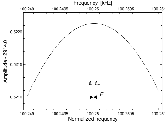
Fig. 1-12. The exponential parabolic interpolation (1-22) on bins 99, 100 and 101 of the magnitude spectrum of Fig. 1-5. The interpolation error E is 19 mHz, i.e. 19 ppm of \Delta_f , and the relative error e amounts to 0.19 ppm. The interpolation decreased the error of 250 Hz of the simple estimate \Delta_f k_m by a factor of 13400. The exponential parabola (1-20) coefficients are \varphi_{me} = 100.250019 , a_e = -0.06319 , h_e = 1.981 and p = 0.085685 .
