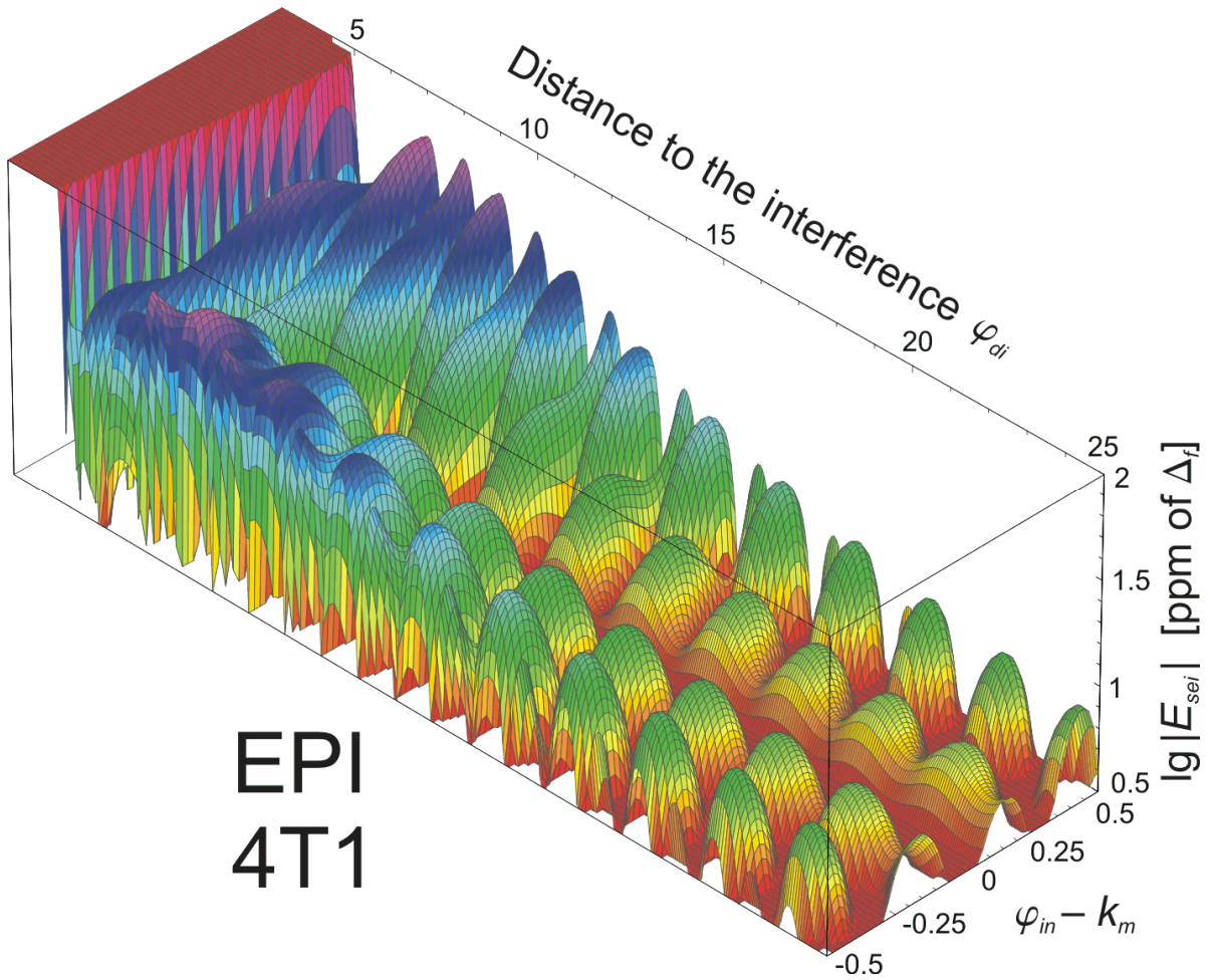
Fig. 4-21. The interpolation systematic error of the EPI method with the 4T1 window as a function of the distance to the interference \varphi_{di} (of the same amplitude as the analyzed component) and the position between two spectrum bins \varphi_d = \varphi_{in} - k_{in} . Note that the interpolation error magnitude is shown on the (decimal) logarithmic scale.
