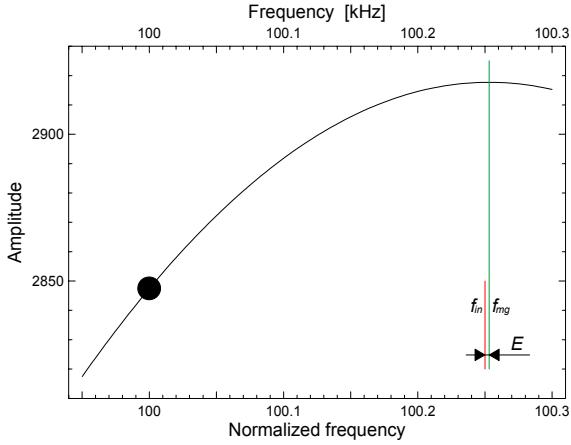
Fig. 1-10. The Gaussian interpolation (1-19) on bins 99, 100 and 101 of the magnitude spectrum of Fig. 1-5. The interpolation error E is 3.1 Hz, i.e. 0.31 % of \Delta_f , and the relative error e amounts to 31 ppm. The Gaussian interpolation decreased the error of 250 Hz of the simplest estimate \Delta_f k_m by a factor of 81. The Gaussian shape (1-17) coefficients are \varphi_{mg} = 100.2531 , a_g = -0.3807 and h_g = 7.978 .
