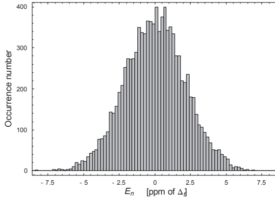
Fig. 4-4. Histogram of the amplitude distribution of the interpolation noise error E_n of Fig. 4-3. The horizontal axis is symmetrical with respect to 0 with the error maximum value of 8.5 ppm as the extremes. The vertical axis is scaled in occurrence numbers for 10000 total cases. Mean and standard deviation values are 7 \times 10^{-3} and 2 ppm of \Delta_f respectively.
