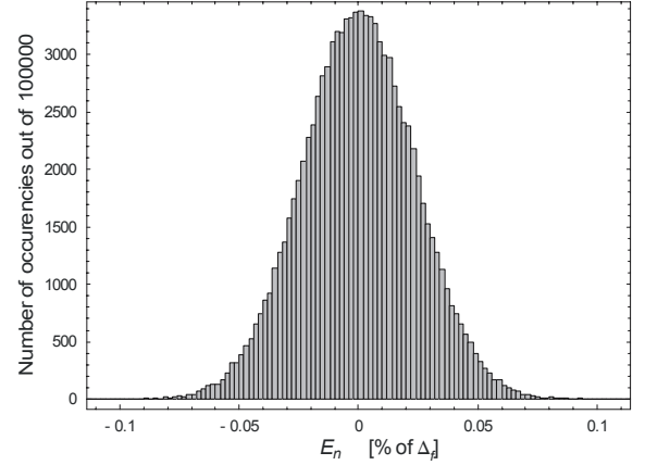
b2) Histogram of noise error E_n of the plot to the left. \{E_n\}_{max}=0.112 [% of \Delta_f ], \{E_n\}_{max}/\{E_n\}_{rms}=4.74
