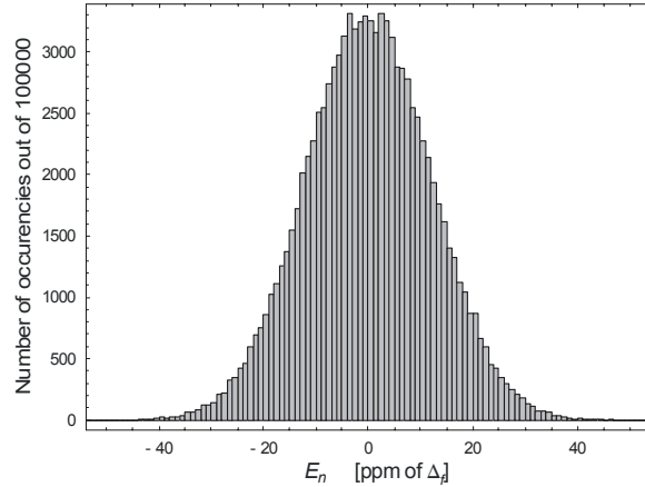
f2) Histogram of noise error E_n of the plot to the left. \{E_n\}_{max} = 53.5 [ppm of \Delta_f ], \{E_n\}_{max} / \{E_n\}_{rms} = 4.44
