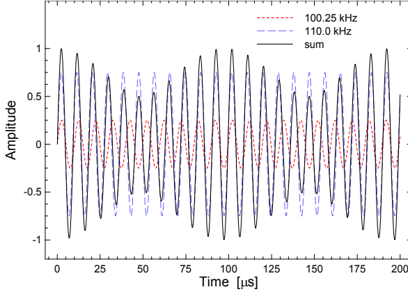
Fig. 1-1. Signal s(t) (black solid line) of unitary amplitude contains two sinusoidal components: the component of interest, s_{in}(t) (red dashed line), whose frequency is to be measured, and an undesirable component, s_{bg}(t) (blue dashed line), considered as a simplified background. Component frequencies are f_{in}=100.25 kHz and f_{bg}=110.0 kHz, their amplitudes A_{in}=0.25 and A_{bg}=0.75 .
