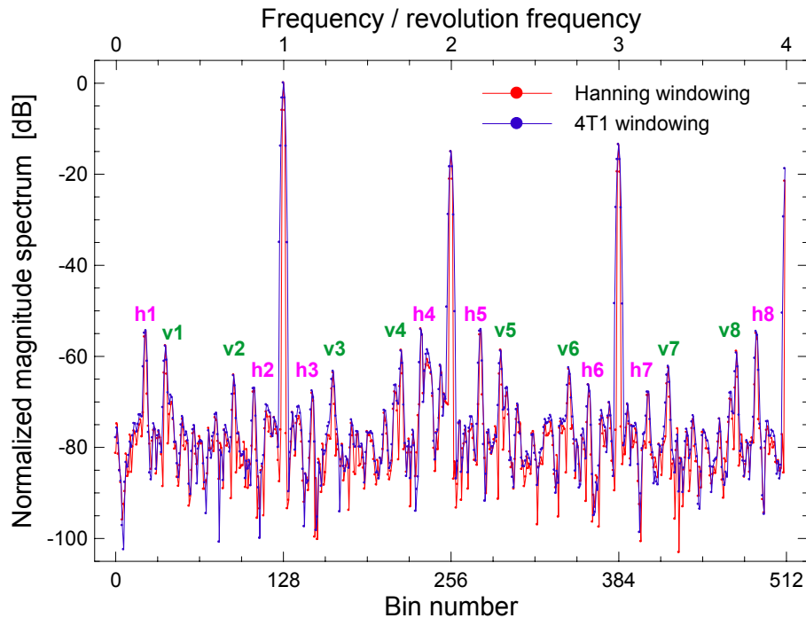
Fig. 5-17. The magnitude spectra of the signal of the above Fig. 5-16, with Hanning and 4T1 windows applied prior to the spectra calculation. Betatron peaks marked with “h” correspond to betatron oscillations in the horizontal machine plane, and these marked with “v” – to the vertical machine plane. This is how looks like a typical spectrum yielded by a tune measurement system of a hadron machine with an important revolution frequency swing.
