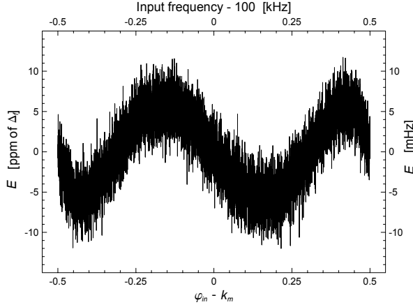
Fig. 4-1. Simulation results of the interpolation error of the EPI method as a function of the shifted DFT input frequency \varphi_{in} - k_m . The error is composed of the systematic part E_s and superimposed noise part E_n , corresponding to the effective resolution of 14 bits. The systematic and noise error contributions are shown separately in Figures 4-2 and 4-3 respectively. The three figures have same scales.
