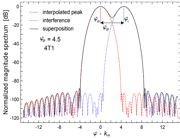
Fig. 4-17. The left spectral peak (of the “superposition spectrum” in black), supposed to be interpolated according to one of the methods studied in this dissertation, is perturbed by a nearby interference, simulated here as a sinusoidal component, giving the right peak. The peaks have equal amplitudes, as the interference is normalized to the amplitude of the component of interest.
