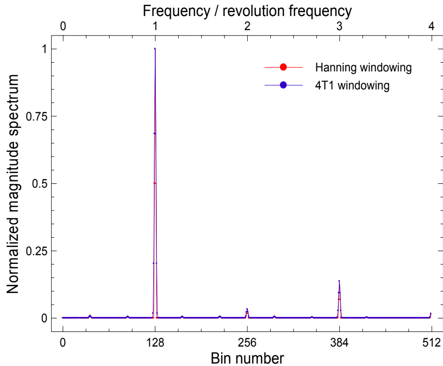
Fig. 5-9. The magnitude spectra of the windowed samples shown in Fig. 5-8. Peaks corresponding to the revolution frequency harmonics are clearly seen and these related to the betatron signal are very small.
