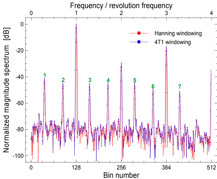
Fig. 5-10. The spectra of the signal of the above Fig. 5-9 in the logarithmic scale. Now the betatron peaks, marked with numbers, are clearly visible. Their amplitudes are some 40 dB (a factor of 100) smaller than the revolution frequency lines and also some 45 dB (a factor of about 180) above the noise floor.
