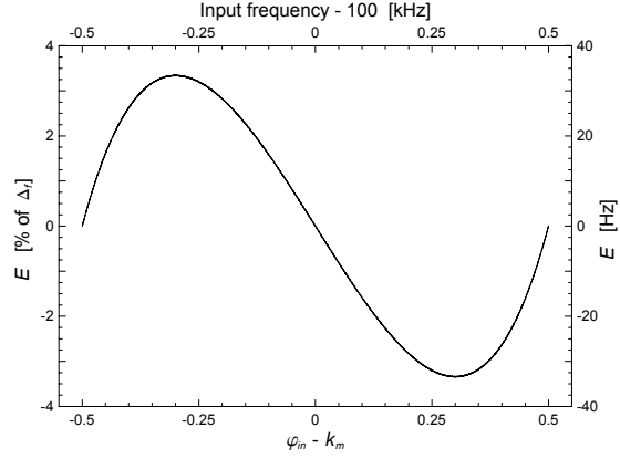
Fig. 1-9. Error E (1-9) of the parabolic interpolation shown in the plot on the left. It is given as a function of the shifted normalized input frequency \varphi_{in} - k_m . The error corresponds directly to the deviation of the curve of Fig. 1-8 from a straight line. The largest error is 3.3 % of \Delta_f for |\varphi_{in} - k_m| = 0.30 , resulting in the interpolation gain (1-16) of 15.
