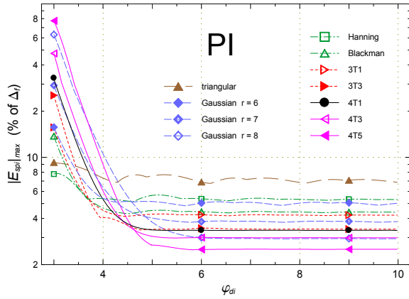
Fig. 4-22. The maximum interpolation systematic error of the PI method for the windows considered in the dissertation as a function of the distance \varphi_{di} to the interference of the same amplitude as the analyzed component.
