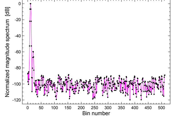
Fig. 2-4. Magnitude spectrum of the time domain sequence shown in the plot on the left. Windowing removed the spectral leakage effect seen in the corresponding plot of Fig. 2-2; please note same scales. It is seen the smaller component of the input sequence as well as noise originating in the quantization of the input samples.
