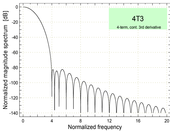
Fig. 2-18. Magnitude spectrum of the weighted cosine window with 4 terms and continuous 3 rd derivative (4T3)
