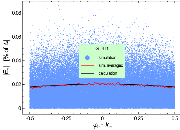
c1) GI method, 4T1 windowing, 2048-points, effective resolution 7.0 bits. \{E_n\}_{rms} from the simulation and calculation [% of \Delta_f ]: 0.0193 and 0.0196, error -1.5 %.
