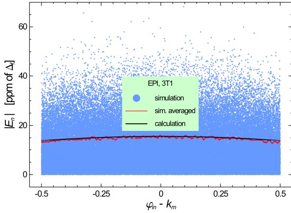
e1) EPI method, 3T1 windowing, 1024-points, effective resolution 11.0 bits. \{E_n\}_{rms} from the simulation and calculation [ppm of \Delta_f ]: 14.7 and 15.0, error -2.0 %.
