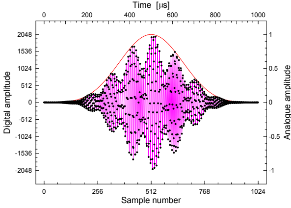
Fig. 1-4. Digitization and windowing of the example input signal. The dots mark N=1024 windowed samples taken with resolution R_c = 12 bits. The red bell-shaped curve is the 4T1 window (1-5).
