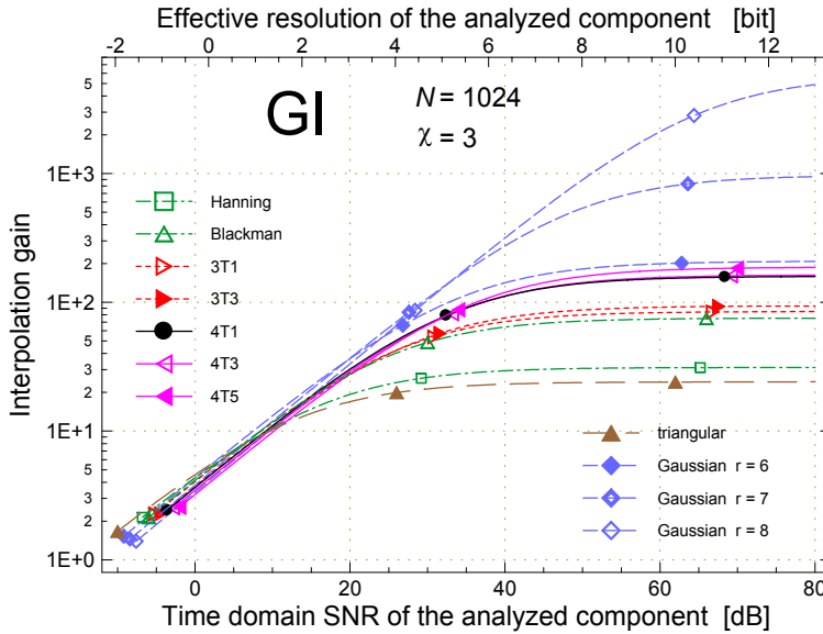
Fig. 4-8. Interpolation gain of the GI method as a function of the time domain SNR of the analyzed component for the windows considered in this dissertation, assuming 1024-point discrete spectra and the noise crest factor \chi of 3.
