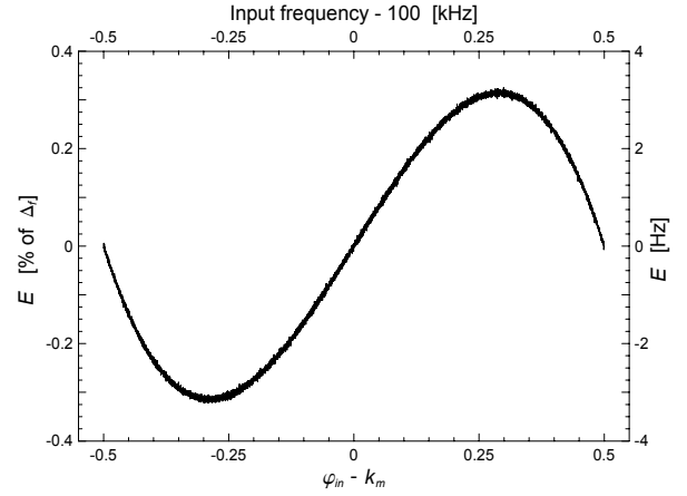
Fig. 1-11. The error (1-9) of the Gaussian interpolation (1-19) as a function of the shifted input frequency \varphi_{in} - k_m . The largest error is 0.33 % of \Delta_f for \varphi_{in} - k_m = 0.30 , resulting in the interpolation gain (1-16) of 150. The noise seen contributes to the interpolation error, decreasing the gain. With no noise, the theoretical gain of the Gaussian interpolation method with the 4T1 windowing is 159, so for this example the influence of the noise seen in the figure is not very important.
