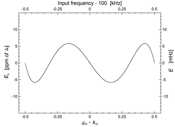
Fig. 4-2. The systematic part E_s of the EPI error E of Fig. 4-1. The largest error is 5.8 ppm of \Delta_f for |\varphi_{in} - k_m| = 0.16 and |\varphi_{in} - k_m| = 0.43 , corresponding to the interpolation gain of 86000.
