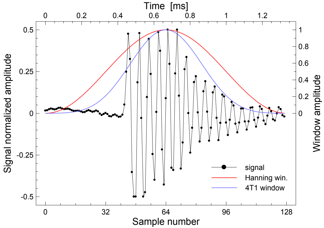
Fig. 5-3. The record of small beam betatron oscillations in the vertical plane of the SPS machine, measured with the BBQ system. The 16-bit samples were taken at the rate of 96 kS/s. The two windows used in the example are also plotted.
