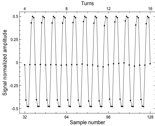
Fig. 5-11. Zoomed samples of Fig. 5-7, revealing the shape of the revolution signal. The shape defines the amplitudes of the revolution harmonic lines seen in Fig. 5-9 and 5-10. The kick was applied to the beam around the middle of the shown record.
