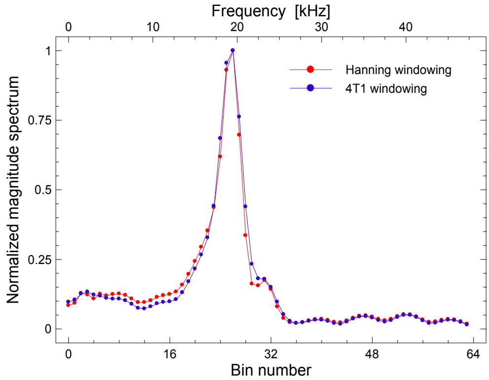
Fig. 5-5. The magnitude spectra of the windowed samples shown in Fig. 5-4.
