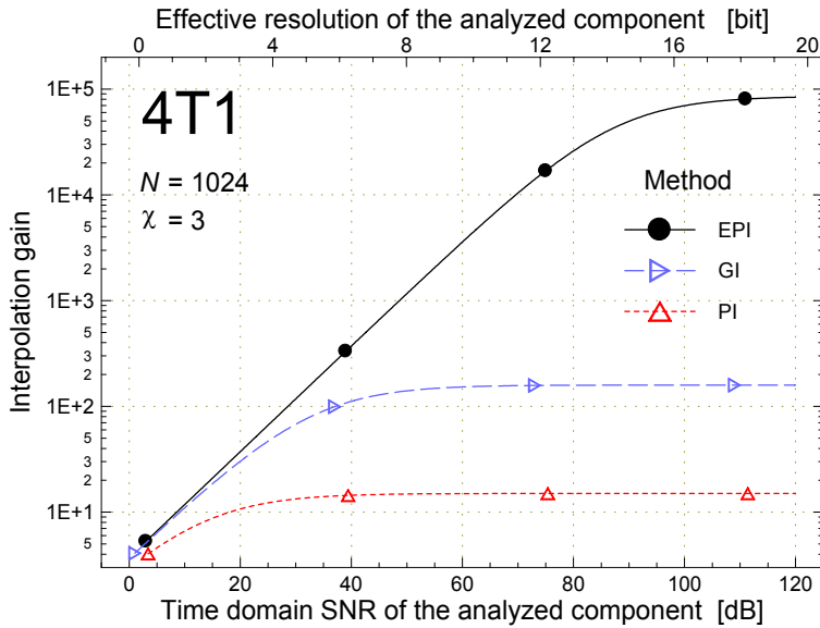
Fig. 4-10. A comparison of the interpolation gain of the three interpolation methods as a function of the time domain SNR of the analyzed component for the 4T1 windowing, 1024-point discrete spectra and the noise crest factor \chi of 3.
