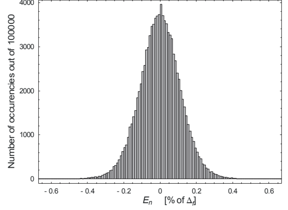
a2) Histogram of noise error E_n of the plot to the left. \{E_n\}_{max}=0.661 [% of \Delta_f ], \{E_n\}_{max}/\{E_n\}_{rms}=5.89
