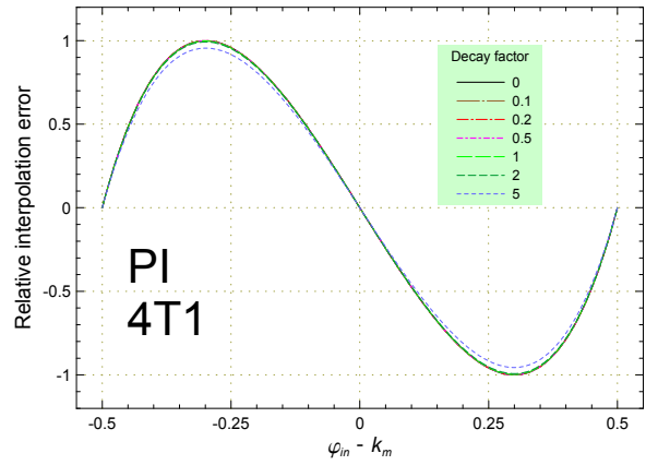
Fig. 4-31. Systematic interpolation error of the PI method with 4T1 window for a few decay factor values.
