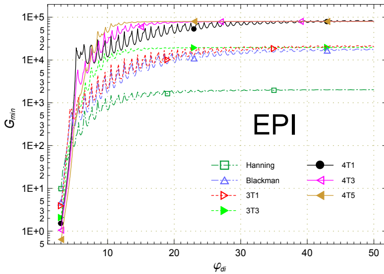
Fig. 4-27b. The minimum interpolation gain of the EPI method for the windows with a fast sidelobe fall-off as a function of the distance \varphi_{di} to the interference of the same amplitude as the analyzed component.
