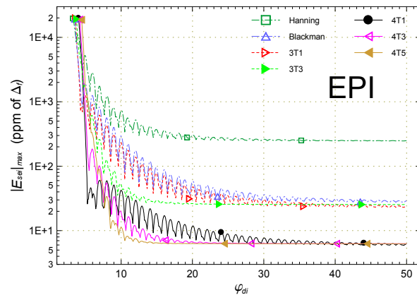
Fig. 4-24b. The maximum interpolation systematic error of the EPI method for the windows with a fast sidelobe fall-off as a function of the distance \varphi_{di} to the interference of the same amplitude as the analyzed component.
