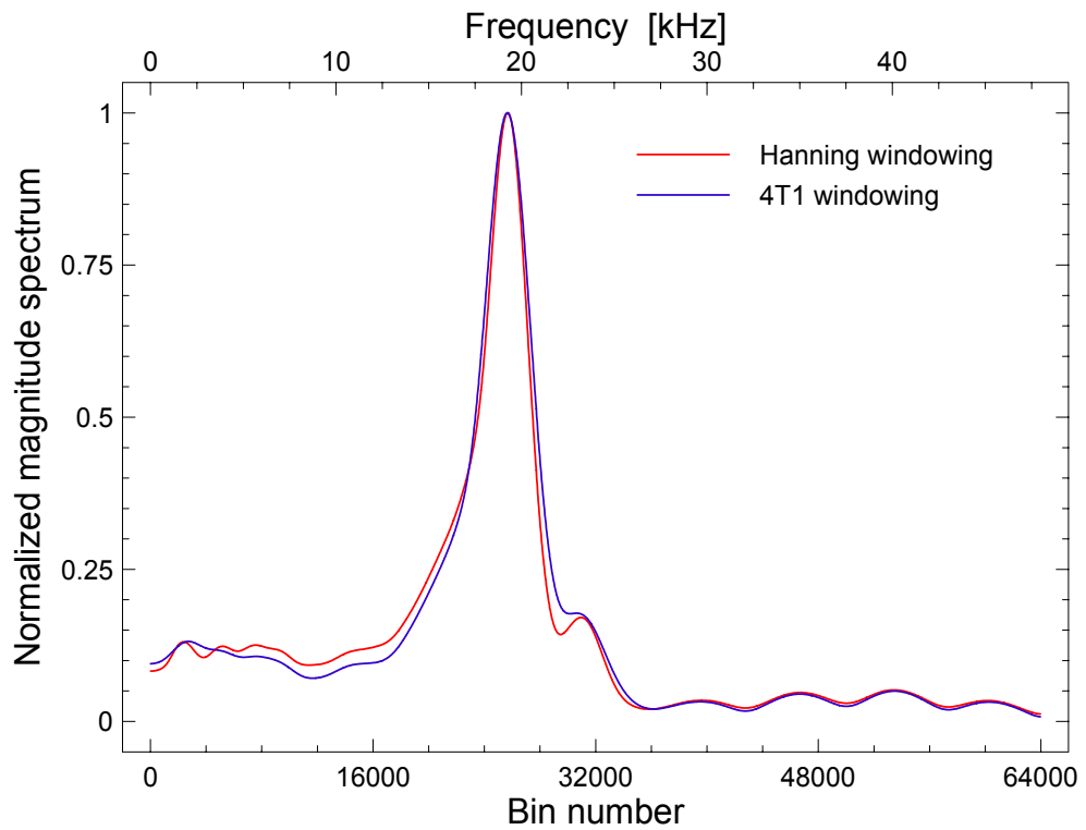
Fig. 5-6. Magnitude spectra of the zero-padded signals, created by extending the 128 sample records of Fig. 5-4 to the length of 128 thousand samples. The spectra are high resolution versions of the spectra of Fig. 5-5 and they are used to estimate the exact values of the betatron frequencies to determine the efficiency of the interpolation methods applied to the low resolution 128-point spectra.
