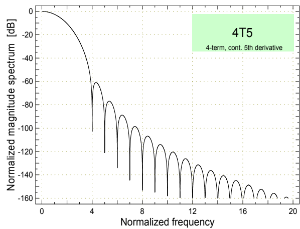
Fig. 2-19. Magnitude spectrum of the weighted cosine window with 4 terms and continuous 5 th derivative (4T5)
