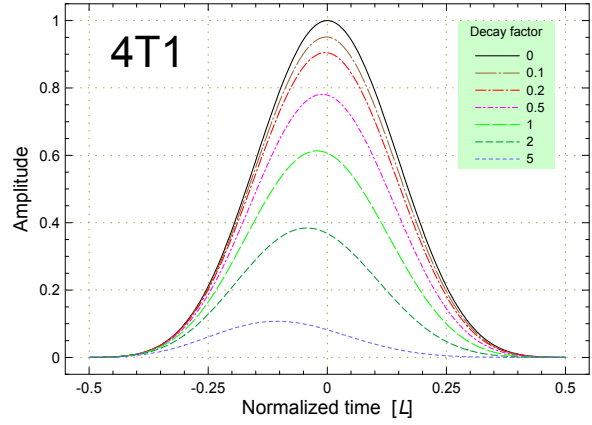
Fig. 4-29. 4T1 window with exponentially decaying functions of Fig. 4-28 superimposed.
