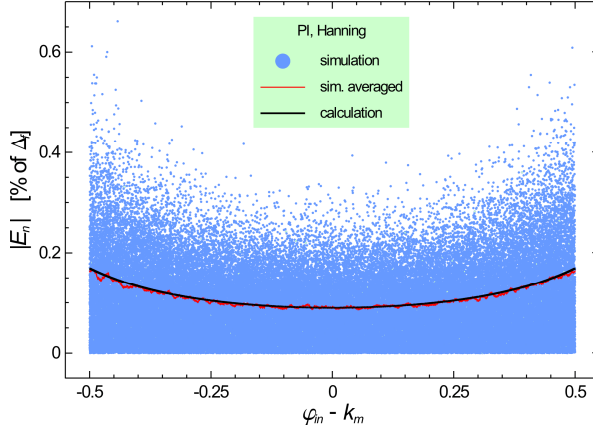
a1) PI method, Hanning windowing, 512-points, effective resolution 5.0 bits. \{E_n\}_{rms} from the simulation and calculation [% of \Delta_f ]: 0.112 and 0.114, error -1.7 %.
