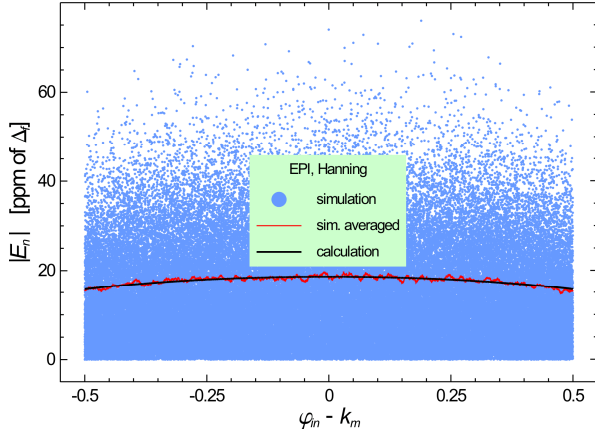
d1) EPI method, Hanning windowing, 512-points, effective resolution 11.0 bits. \{E_n\}_{rms} from the simulation and calculation [ppm of \Delta_f ]: 17.8 and 17.7, error 0.6 %.
