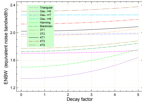
Fig. 4-37. The ENBW of particular windows as a function of the decay factor.
