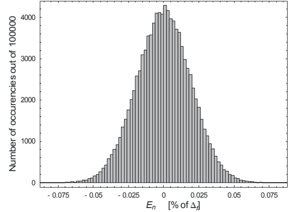
c2) Histogram of noise error E_n of the plot to the left. \{E_n\}_{max}=0.0864 [% of \Delta_f ], \{E_n\}_{max}/\{E_n\}_{rms}=4.48
