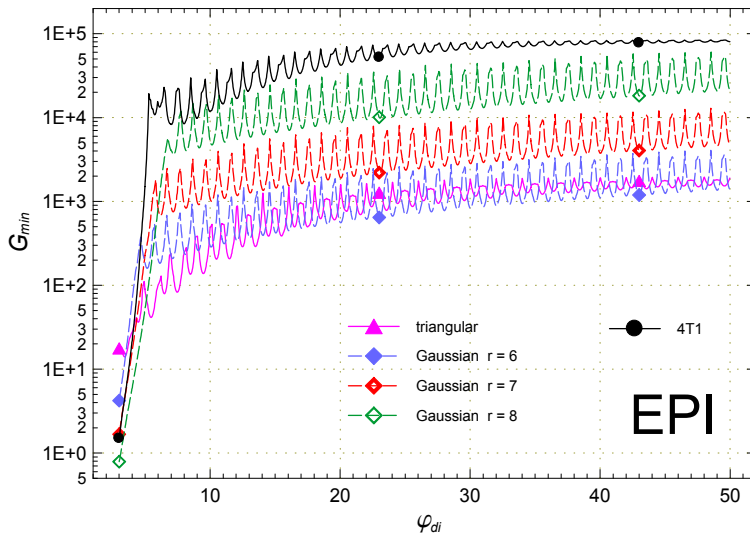
Fig. 4-27a. The minimum interpolation gain of the EPI method for the windows with a slow sidelobe fall-off as a function of the distance \varphi_{di} to the interference of the same amplitude as the analyzed component. The case of the 4T1 window, having a fast sidelobe decay, is shown as a reference and a link to the plot below, displaying the gain for the windows with a fast sidelobe fall-off. The two plots have same scales.
