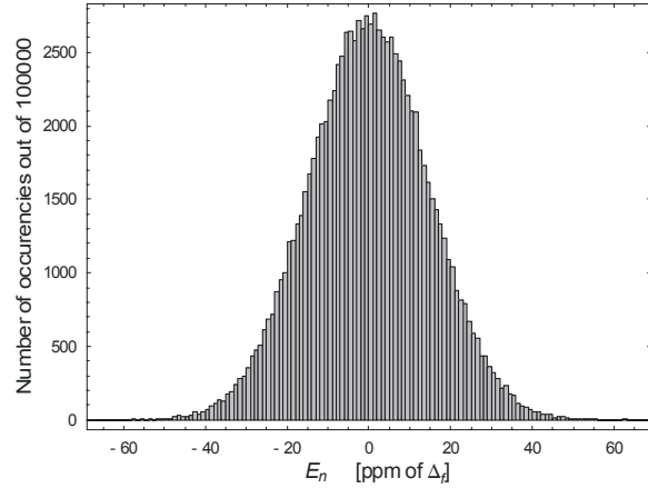
e2) Histogram of noise error E_n of the plot to the left. \{E_n\}_{max} = 68.2 [ppm of \Delta_f ], \{E_n\}_{max} / \{E_n\}_{rms} = 4.65
