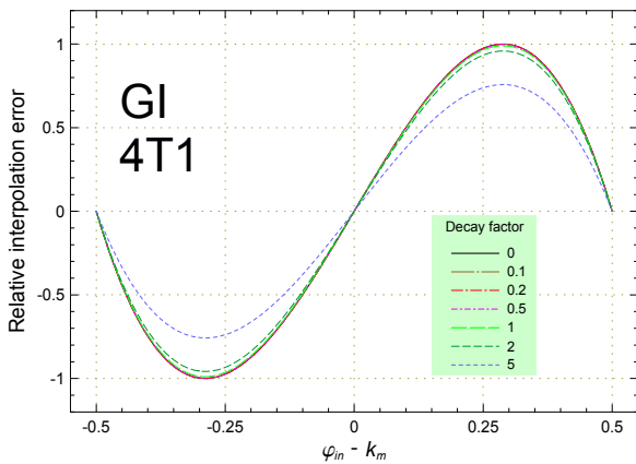
Fig. 4-32. Systematic interpolation error of the GI method with 4T1 window for a few decay factor values.
