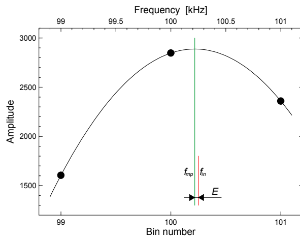
Fig. 1-6. Parabolic interpolation (1-12) on the bins 99, 100 and 101 of the magnitude spectrum of Fig. 1-5. The interpolation error E is -32 Hz, i.e. 3.2 % of \Delta_f and the relative error e amounts to -0.07 %. The parabolic interpolation decreased the error of 250 Hz of the simple estimate \Delta_f k_m by a factor of 7.8. The coefficients of parabola (1-11) are f_{mp} = 100.2180 , a_p = -865.3 and h_p = 2888.5 .
