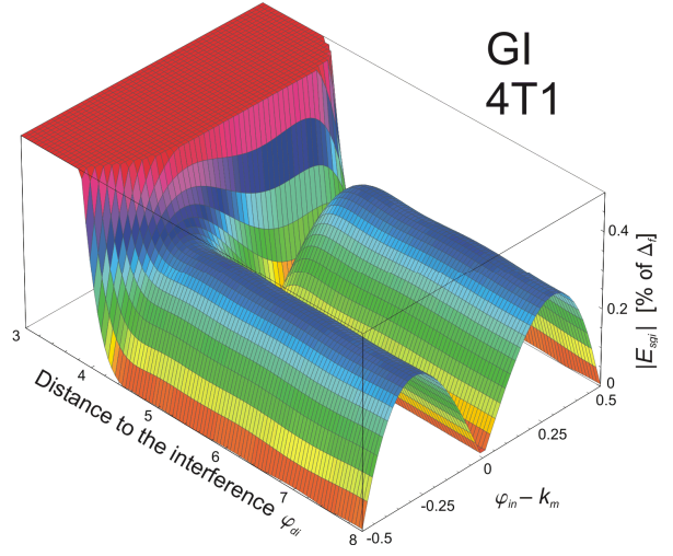
Fig. 4-20. The interpolation systematic error of the GI method with the 4T1 window as a function of the distance to the interference \varphi_{di} (of the same amplitude as the analyzed component) and the position between two spectrum bins \varphi_d = \varphi_{in} - k_{in} .
