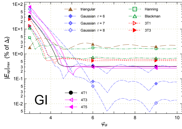
Fig. 4-23. The maximum interpolation systematic error of the GI method for the windows considered in the dissertation as a function of the distance \varphi_{di} to the interference of the same amplitude as the analyzed component.
