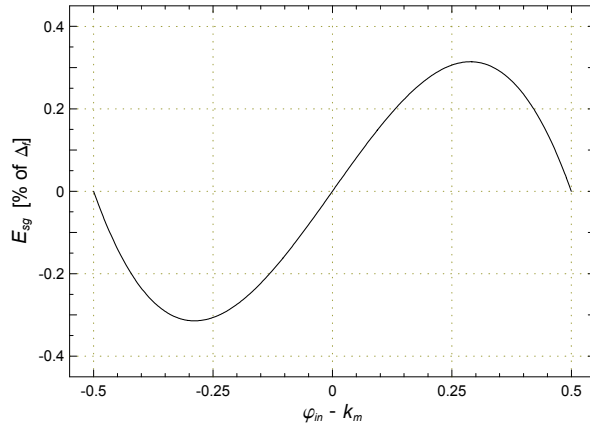
Fig. 3-4. The systematic error of the Gaussian interpolation for 4T1 windowing. Its maximum value is 0.31 % of \Delta_f for |\varphi_d| = 0.29 ; the corresponding interpolation gain is 159. The errors for other windows have similar shapes and can be characterized by the error maximum E_{max} = \max(|E_{sg}(\varphi_d)|) and its abscissae. They are listed in Table 3-3.
