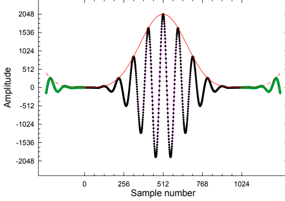
Fig. 2-3. Sample sequence (2.3-1) (black dots and magenta line) windowed with the 4T1 window (red line) and their replicas (green line for the sequence and dashed red line for the window).
