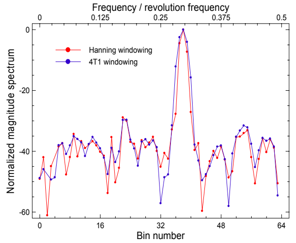
Fig. 5-15. The magnitude spectra of Fig. 5-14 in the logarithmic scale.
