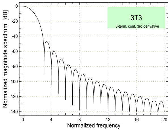
Fig. 2-16. Magnitude spectrum of the weighted cosine window with 3 terms and continuous 3 rd derivative (3T3).
