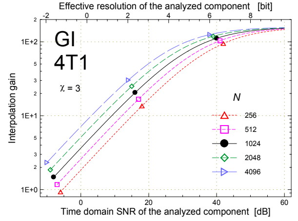
Fig. 4-12. The interpolation gain of the GI method as a function of the discrete spectrum bin number N , assuming the 4T1 windowing and the noise crest factor \chi of 3.
