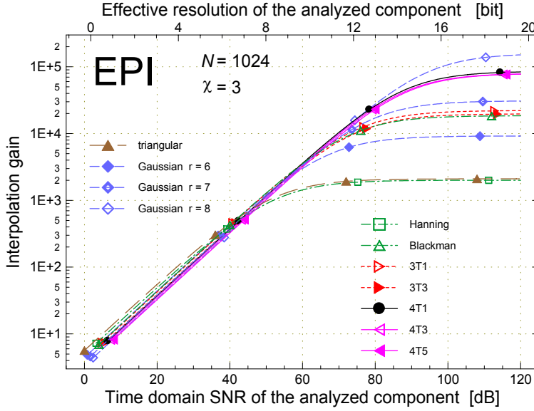
Fig. 4-7. Interpolation gain of the EPI method as a function of the time domain SNR of the analyzed component for the windows considered in this dissertation, assuming 1024-point discrete spectra and the noise crest factor \chi (4.1-22) of 3.
