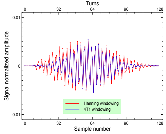
Fig. 5-13. The samples of Fig. 5-12 windowed according to the Hanning and 4T1 functions.
