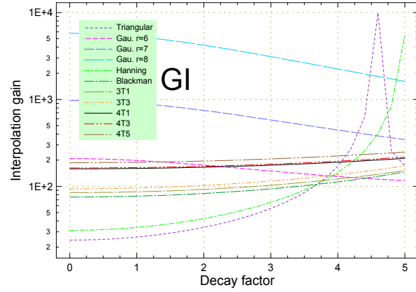
Fig. 4-35. Minimal interpolation gain of the GI method as a function of the decay factor.
