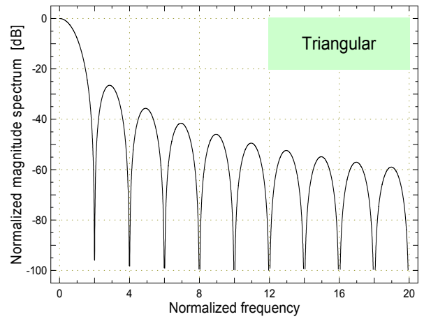
Fig. 2-9. Magnitude spectrum of the triangular window.
