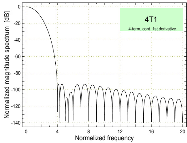
Fig. 2-17. Magnitude spectrum of the weighted cosine window with 4 terms and continuous 1 st derivative (4T1)
