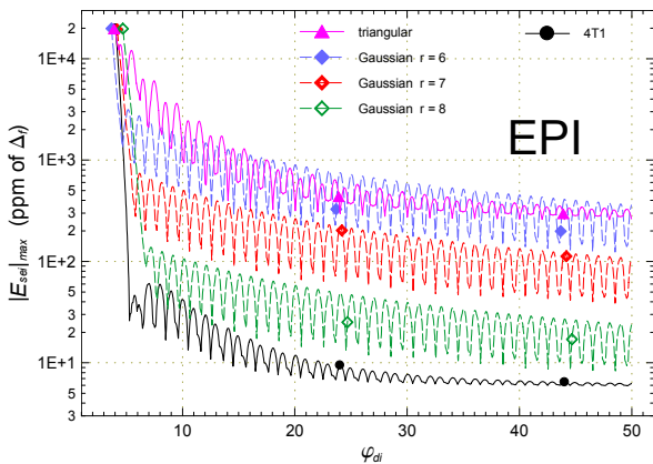
Fig. 4-24a. The maximum interpolation systematic error of the EPI method for the windows with a slow sidelobe fall-off as a function of the distance \varphi_{di} to the interference of the same amplitude as the analyzed component. The case of the 4T1 window, having a fast sidelobe decay, is shown as a reference and a link to the plot on the right, displaying the error for the windows with a fast sidelobe fall-off. The two plots have same scales.
