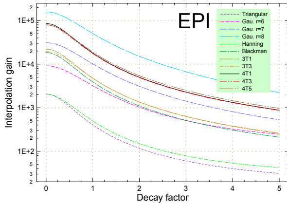
Fig. 4-36. Minimal interpolation gain of the EPI method as a function of the decay factor.
