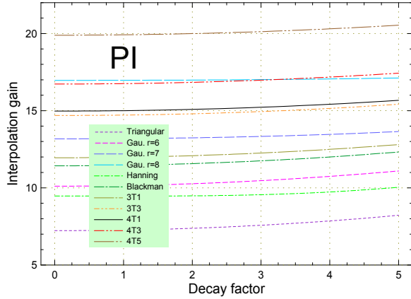
Fig. 4-34. Minimal interpolation gain of the PI method as a function of the decay factor.
