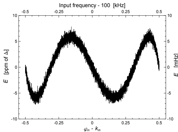
Fig. 1-14. The error E (1-9) of the exponential parabolic interpolation as a function of the shifted DFT input frequency \varphi_{in} - k_m . The error is composed of the systematic part and a superimposed noise part, corresponding to the effective resolution of 16 bits. The largest error is -7.8 ppm of \Delta_f for \varphi_{in} - k_m = 0.156 , resulting in the interpolation gain (1-16) of 63800. These are the worst values from 10000 simulation results seen on the figure.
