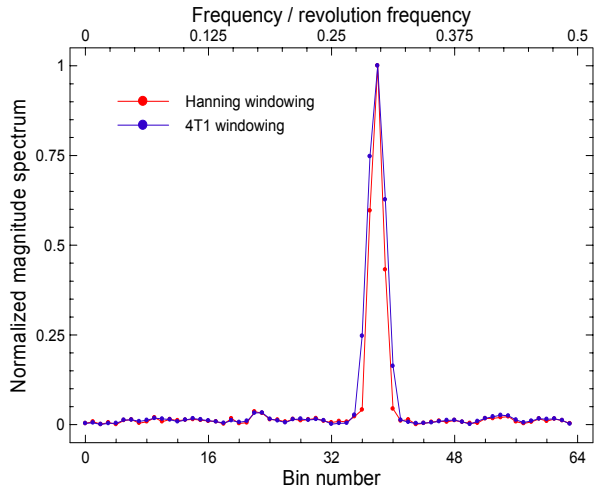
Fig. 5-14. The magnitude spectra of the windowed samples shown in Fig. 5-13. The large peak corresponds to the vertical plane betatron frequency.
