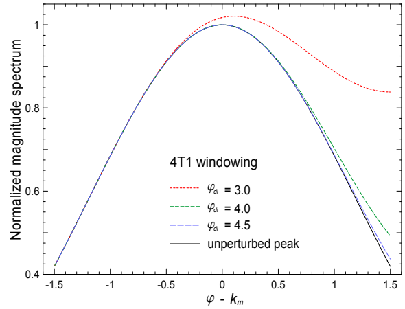
Fig. 4-18. Shapes of the interference-perturbed spectral peak for 4T1 windowing. In the plot three interference locations are considered: 3, 4 and 4.5 bins from the frequency of the component of interest. The shape of the unperturbed peak is given for a comparison (solid black curve).
