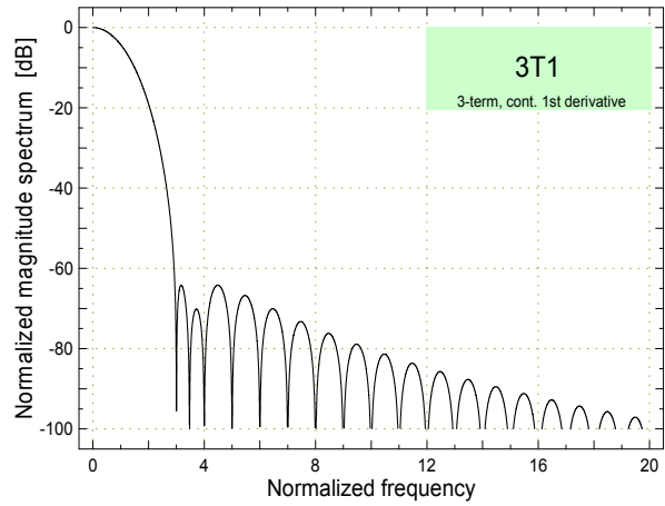
Fig. 2-15. Magnitude spectrum of the weighted cosine window with 3 terms and continuous 1 st derivative (3T1).
