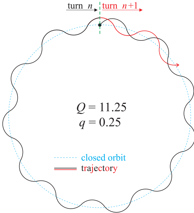
Fig. 5-1. The concept of the betatron tune of an accelerator and betatron resonance. The tune value Q is the number of betatron oscillation periods per machine revolution and q is its fractional part. If q is a quotient of small integers then every a few turns the betatron oscillations have the same phase in a given machine point and in such conditions they can build up until the beam is lost. On the sketch q=0.25 , i.e. every four turns the betatron oscillations superimpose on themselves and the oscillation amplitude may grow.
