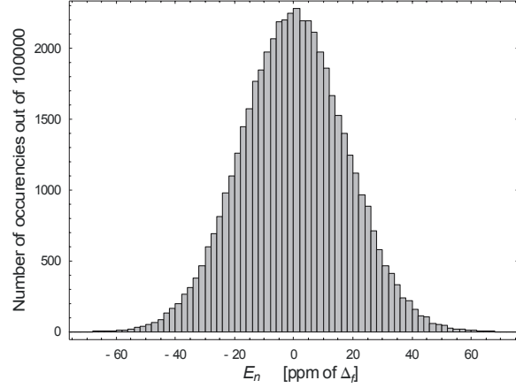
d2) Histogram of noise error E_n of the plot to the left. \{E_n\}_{max} = 76.0 [ppm of \Delta_f ], \{E_n\}_{max} / \{E_n\}_{rms} = 4.27
