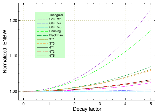
Fig. 4-38. The normalized ENBW of particular windows as a function of the decay factor.
