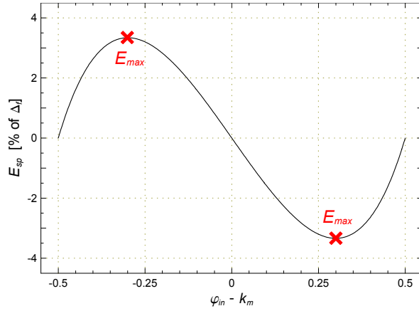
Fig. 3-2. The systematic error of the parabolic interpolation for 4T1 windowing. Its maximum value is 3.3 % of \Delta_f for |\varphi_d|=0.3 ; the corresponding interpolation gain is 15. The errors for other windows have similar shapes and can be characterized by the error maximum E_{max} = \max(|E_{sp}(\varphi_d)|) and its abscissae. They are listed in Table 3-2.
