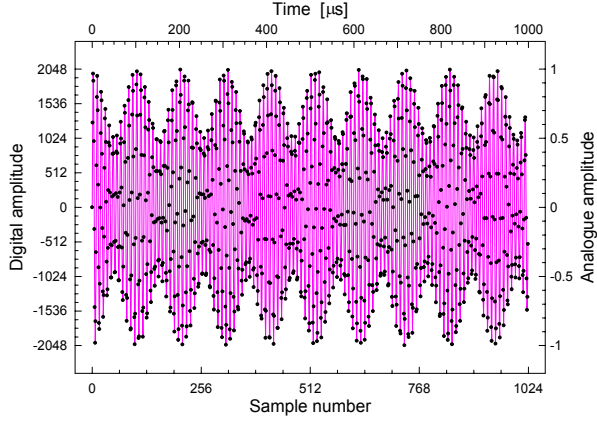
Fig. 1-2. Digitization of the example input signal. The dots mark the samples taken with the converter resolution R_c = 12 bits and the sampling rate f_s = 1.024 MHz. About hundred periods of the signal input component are acquired. The signal envelope results from beating of the input and background components.
