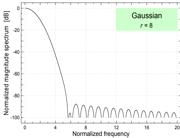
Fig. 2-12. Magnitude spectrum of the Gaussian window of length 8\sigma (i.e. truncated at \pm 4\sigma ).
