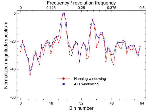
Fig. 5-19. The magnitude spectra of the windowed signal of Fig. 5-18. The left (larger) peak corresponds to the betatron oscillations in the horizontal plane, and the right (smaller) one – to the oscillations in the vertical plane.
