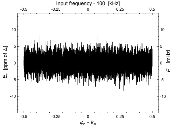
Fig. 4-3. The noise part E_n of the EPI error E of Fig. 4-1. The largest error is 8.5 ppm of \Delta_f for \varphi_{in} - k_m = 0.08 , as the worst case from 10000 simulations seen on the figures. The noise error is an important contribution to the total noise seen in Fig. 4-1.
