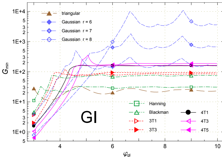
Fig. 4-26. The minimum interpolation gain of the GI method for the windows considered in the dissertation as a function of the distance \varphi_{di} to the interference of the same amplitude as the analyzed component.
