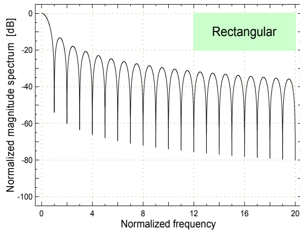
Fig. 2-8. Magnitude spectrum of the rectangular window.
