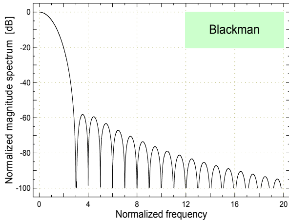
Fig. 2-14. Magnitude spectrum of the Blackman window.
