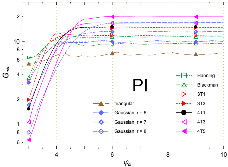
Fig. 4-25. The minimum interpolation gain of the PI method for the windows considered in the dissertation as a function of the distance \varphi_{di} to the interference of the same amplitude as the analyzed component.
