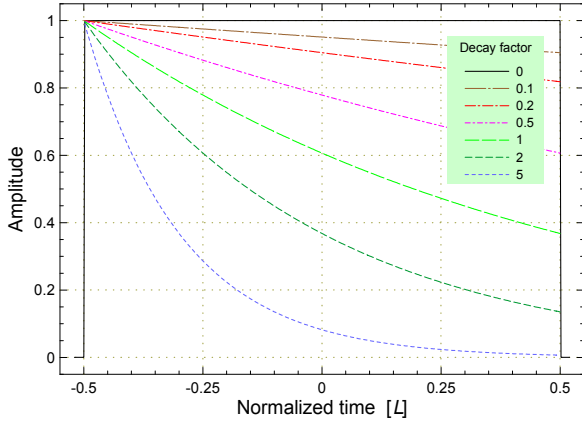
Fig. 4-28. Shapes superimposed on the window functions to simulate exponential decay of the analyzed signal.
