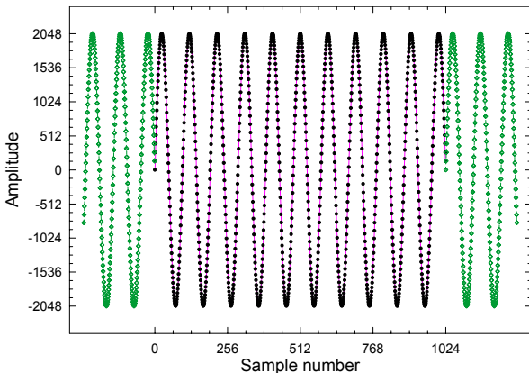
Fig. 2-1. Sample sequence (2.3-1) (black dots and magenta line) and its replicas (dashed line, green) as seen by the DFT.
