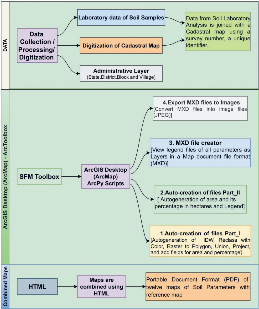
Fig. 8. Architecture of the SFMTtoolbox
