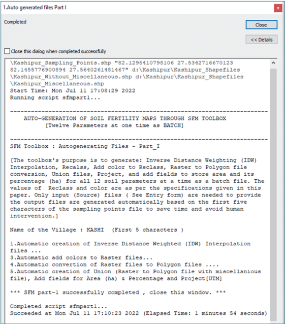
Fig. 12. Execution of ArcPy script of Auto-generated files Part I
