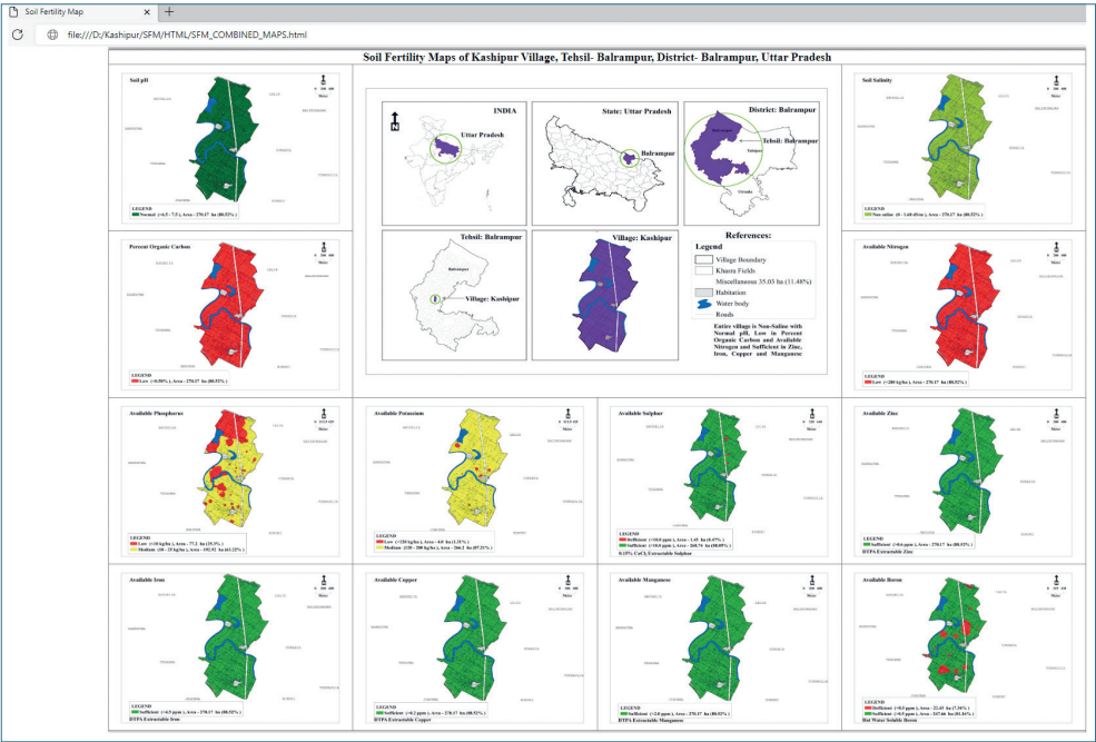
Fig. 27. Twelve parameters soil fertility maps of village – Kashipur, tehsil – Balrampur, district – Balrampur, and state – Uttar Pradesh, India
