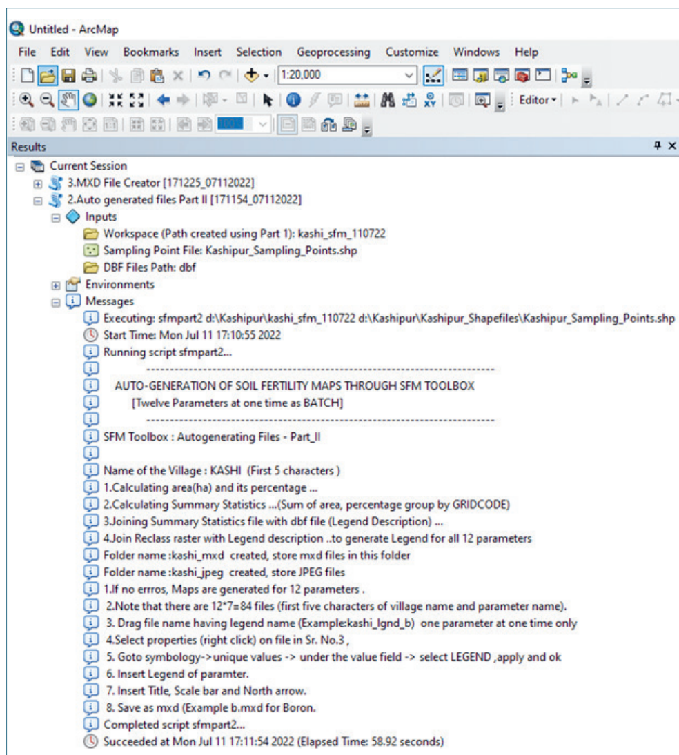
Fig. 16. Results of ArcPy script of Auto-generated files Part II
