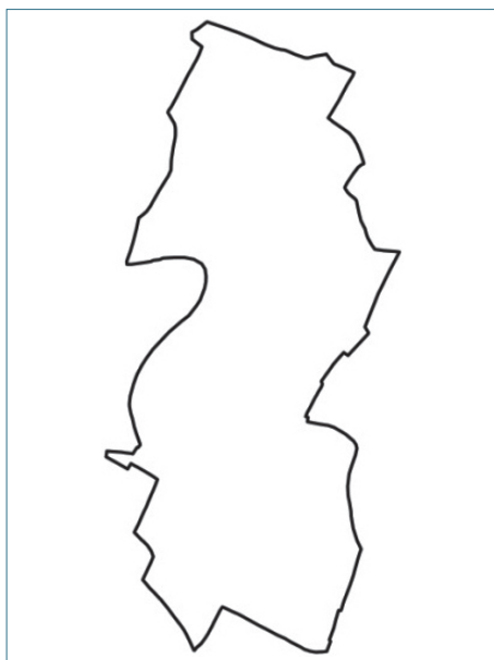
Fig. 6. Village layer outer boundary
