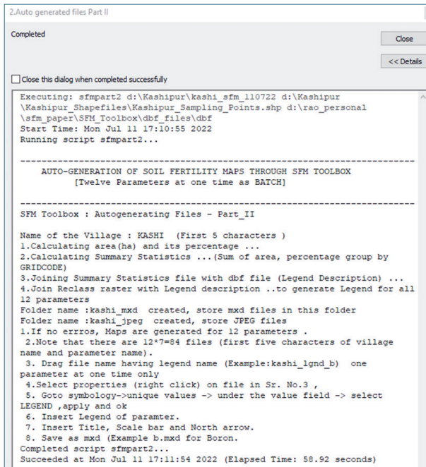
Fig. 15. Execution of ArcPy script of Auto-generated files Part II
