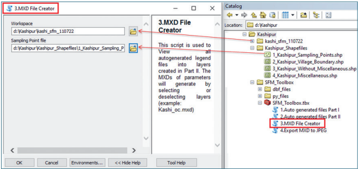
Fig. 19. User interface of MXD File Creator with input files and folders
