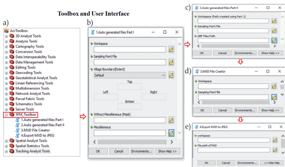
Fig. 10. The user interface of the SFMToolbox: a) tools of SFMToolbox and interfaces; b) Auto-generated files Part I; c) Auto-generated files Part II; d) MXD File Creator; e) Export MXD to JPEG
