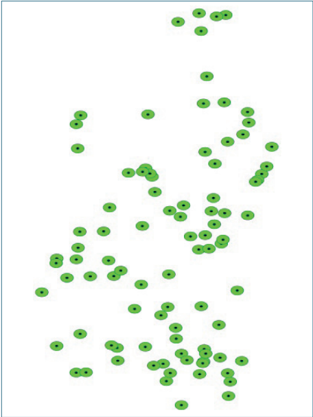
Fig. 4. Sampling points having 12 parameters laboratory data values
