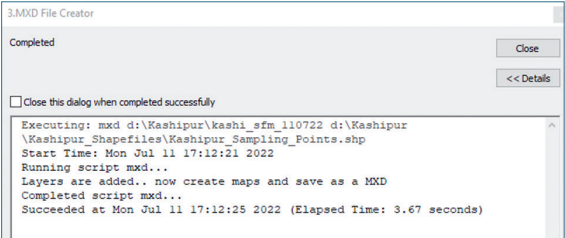
Fig. 20. Execution of ArcPy script of MXD File Creator
