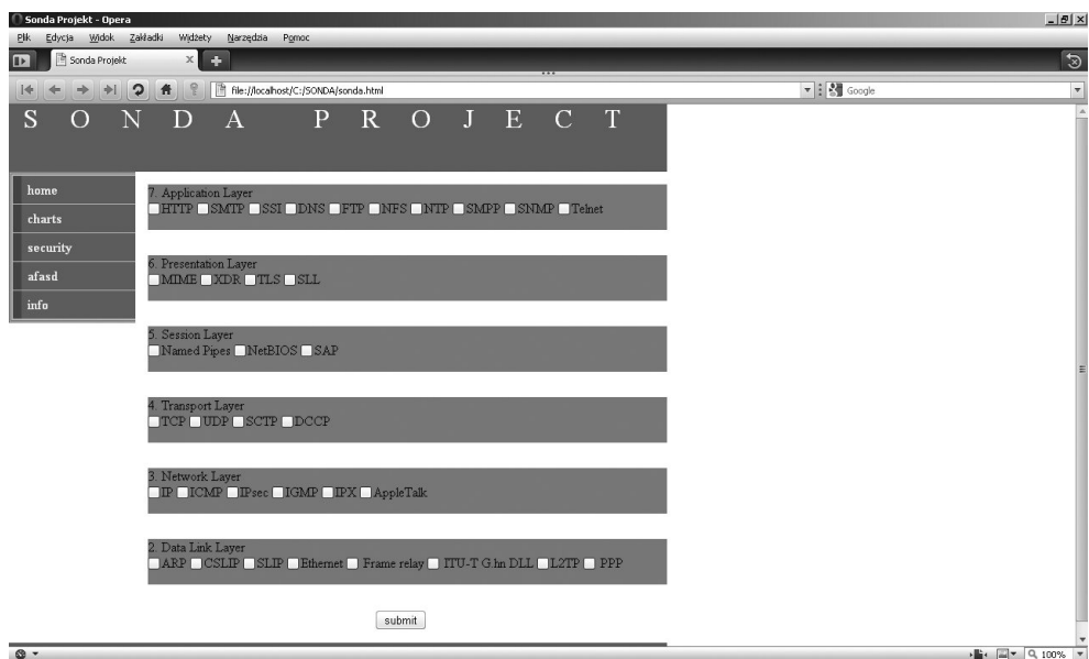
Fig. 6. Program interface
