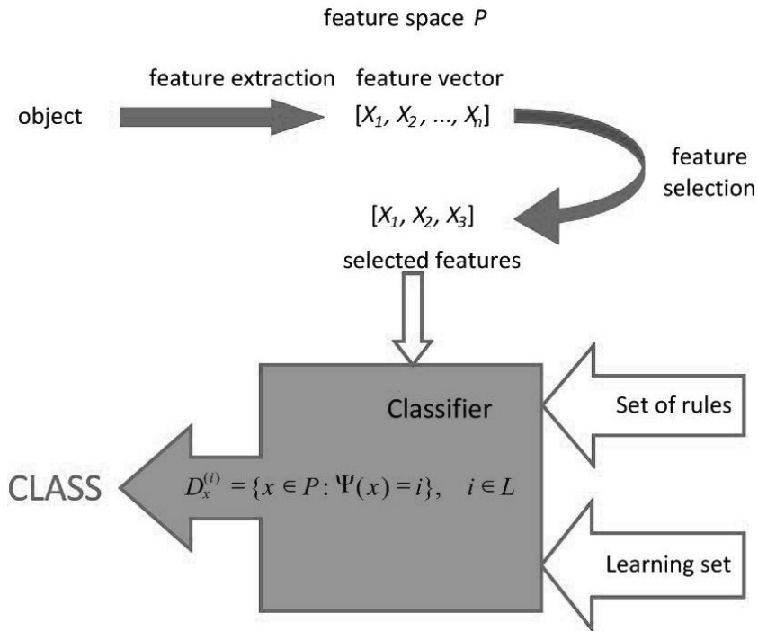
Fig. 4. Supervised classification
