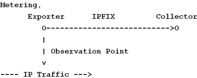
Fig. 2. Anatomy of Simple Network Management Protocol
