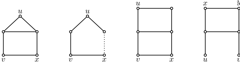
Fig. 2. Graphs: house H , hole H , domino D and A -graph (from left to right)
