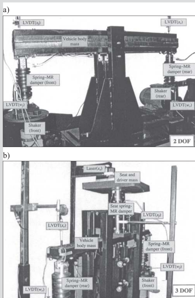
Fig. 3. General view of: 2 DOF experimental setup (a), 3 DOF experimental setup (b)
