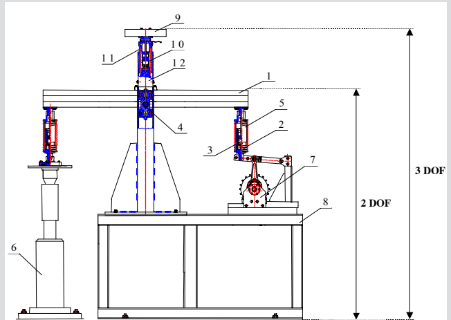
Fig. 2. 2 DOF/3 DOF experimental setup drawing (see text)
