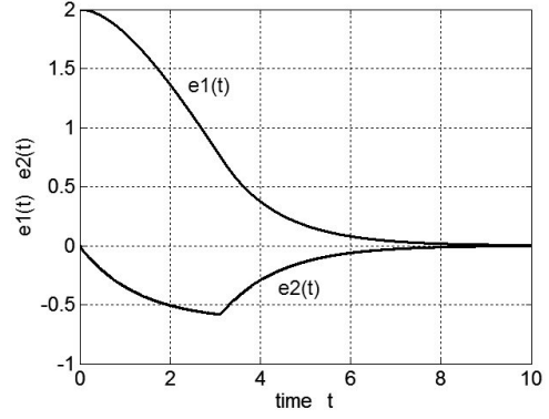
Fig. 3. Tracking error and its derivative (ITAE minimization)
