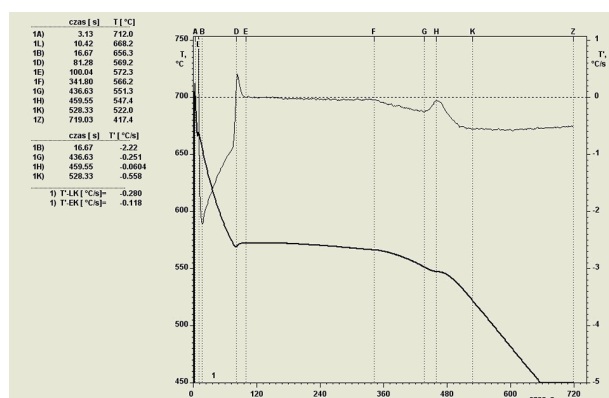
Fig. 4. Thermal-Derivative Analysis (TDA) diagram for silumin AlSi21CuNiMg modified with AlCu19P1.4
