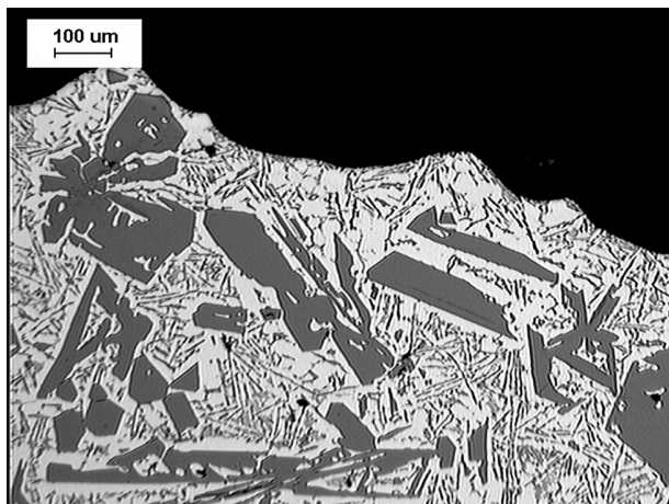
Fig. 13. Microphotography of the profile of the fracture of silumin AlSi21CuNiMg without modification
