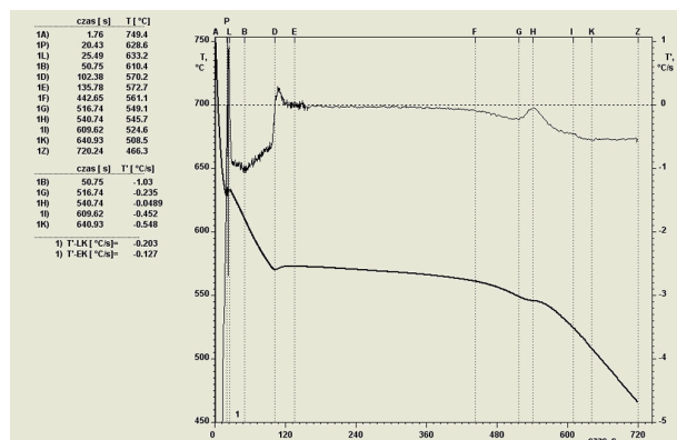
Fig. 3. Thermal-Derivative Analysis (TDA) diagram for silumin AlSi21CuNiMg without modification
