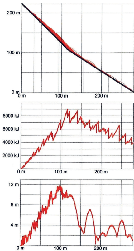
Fig. 7. Envelope curve: total kinetic energy Ec and bounce height (Profile 3)
