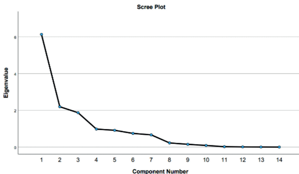
Fig. 22. Scree plot of the Principal Component Analysis
