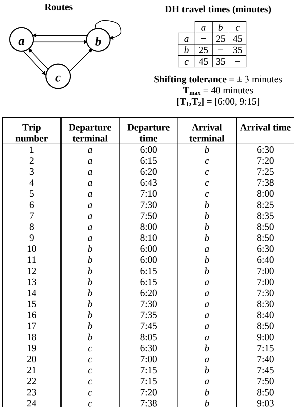
Fig. 7. Example consisting of 24 trips and 3 terminals for constructing vehicle chains with the T_{\max} constraint
