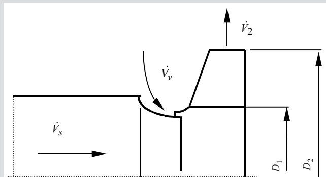
Fig. 4. Consideration of volumetric loss
