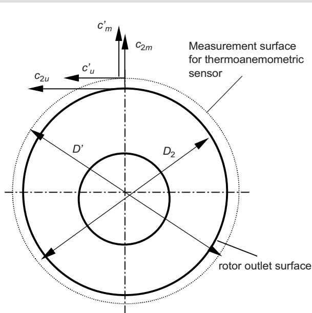
Fig. 3. Velocities at D_2, D' diameters
