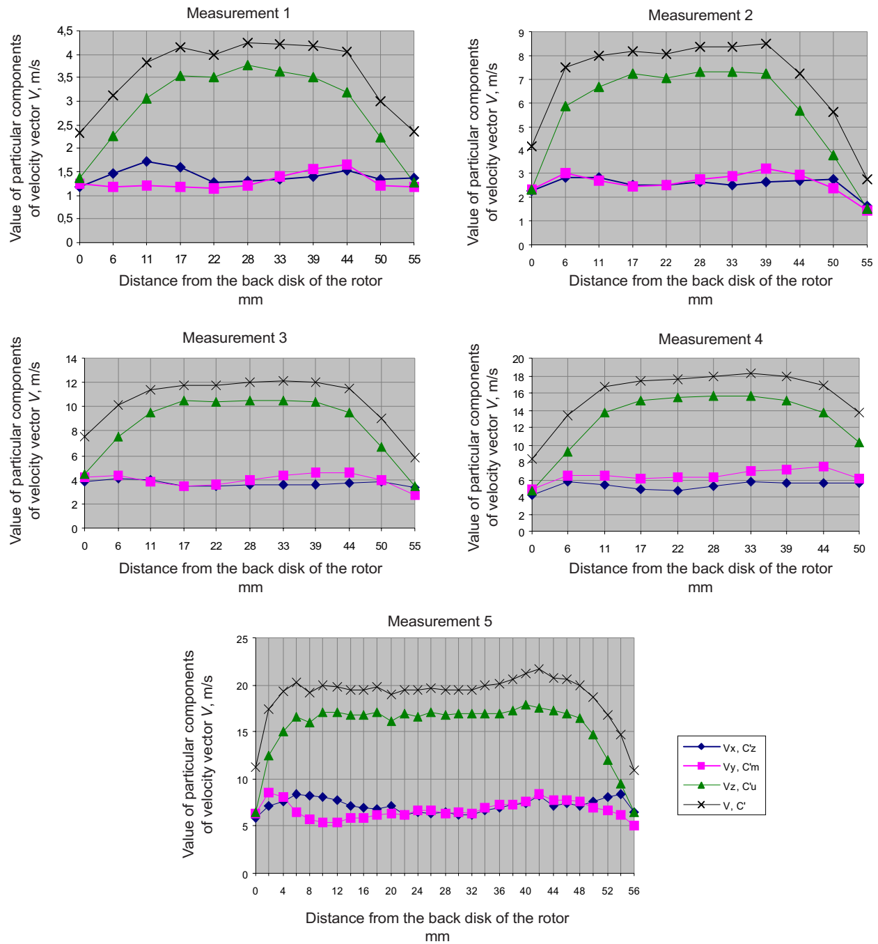
Fig. 2. Velocities measured for revolutions 439(1), 897(2), 1368(3), 2038(4), 2260 r.p.m (5 subsequent from the top). The diagram shows averaging values after rotation time 0–30 ms along the blade width
