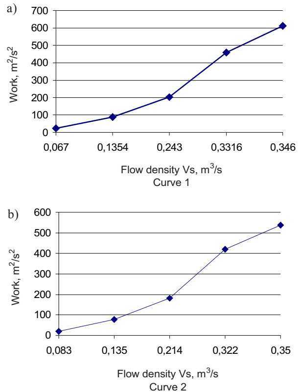
Fig. 5. Comparison of whirl work based on thermoanemometric measurements (a) and balance measurements (b)
