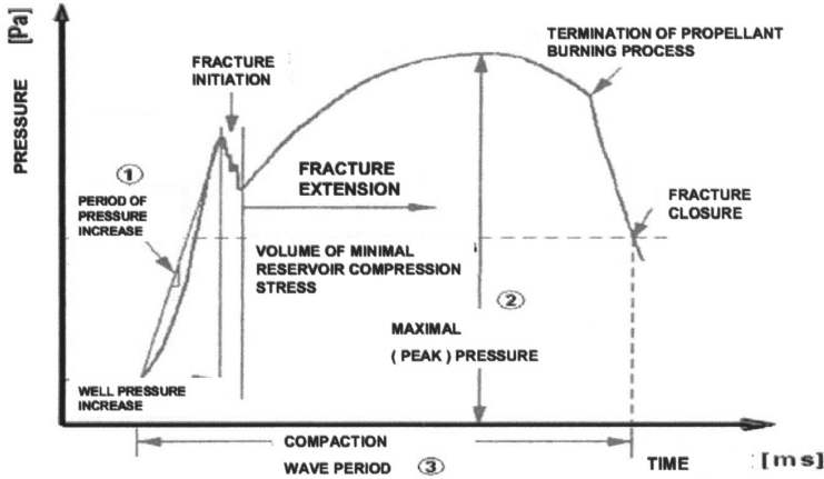
Fig. 4. Typical time-pressure diagram of propellant fracturing process
