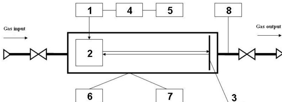
Fig. 2. Functional diagram of block for measuring the sound dispersion speed in gas: 1 – generation-receiving circuit, 2 – primary ultrasound transducer, 3 – reflector, 4 – processing results device, 5 – device output, 6 – humidity sensor, 7 – temperature sensor, 8 – pressure sensor
