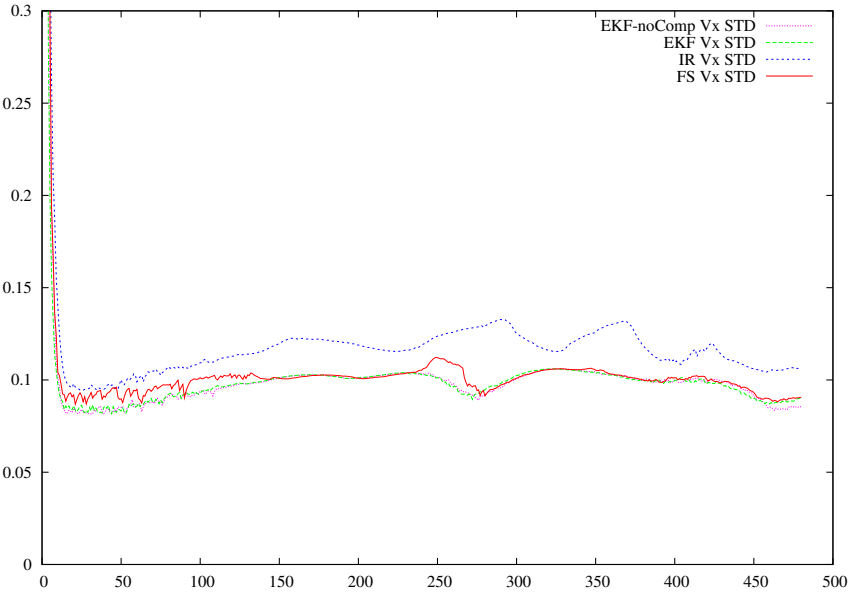
Figure 5.45: Linear velocity standard deviation (X coordinate).
