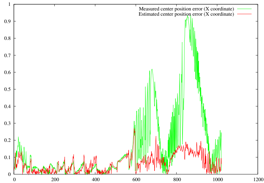
Figure 6.30: Tracked object centre's position error - X coordinate.
