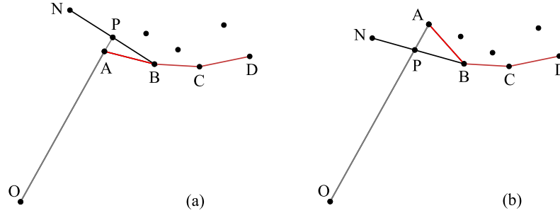
Figure 5.2: Convex-hull construction.
