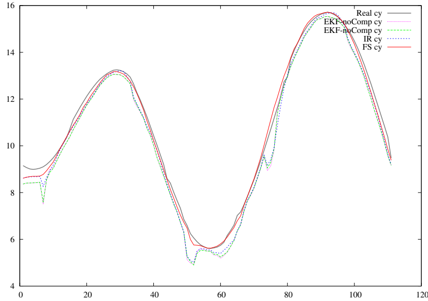
Figure 5.65: Center position estimation (Y coordinate).
