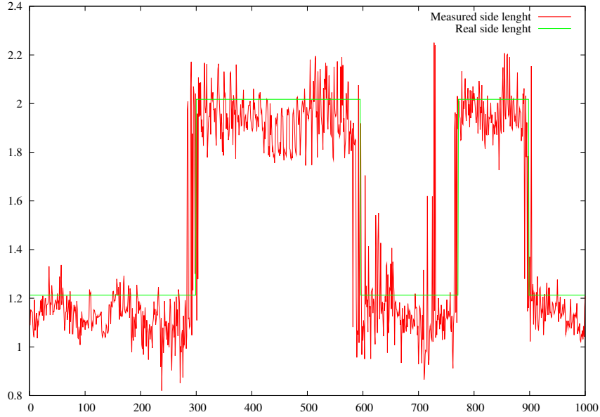
Figure 5.13: The side length measurement (LT, T=1.645 ).
