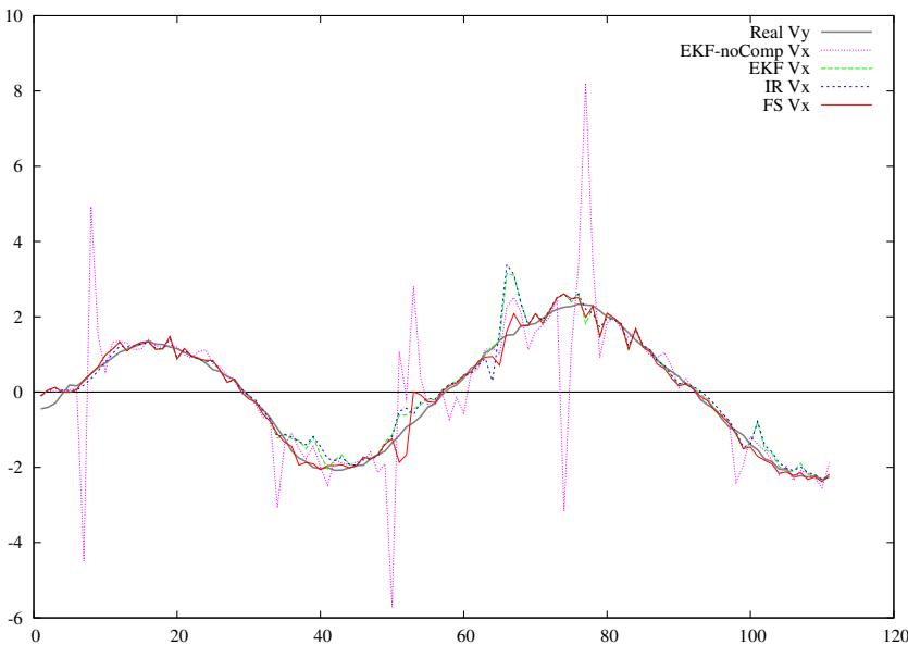
Figure 5.71: Linear velocity estimation (Y coordinate).
