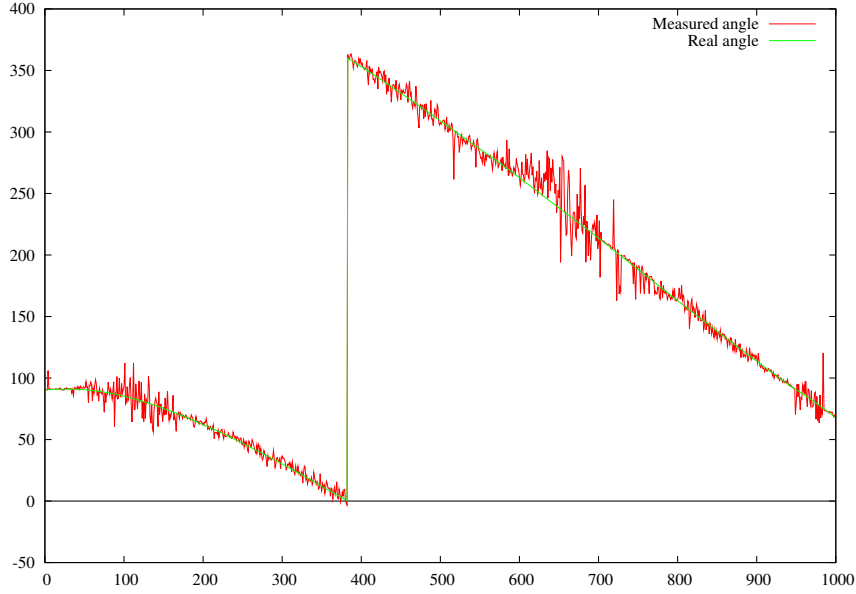
Figure 5.10: Orientation angle measurement (c-Hull).
