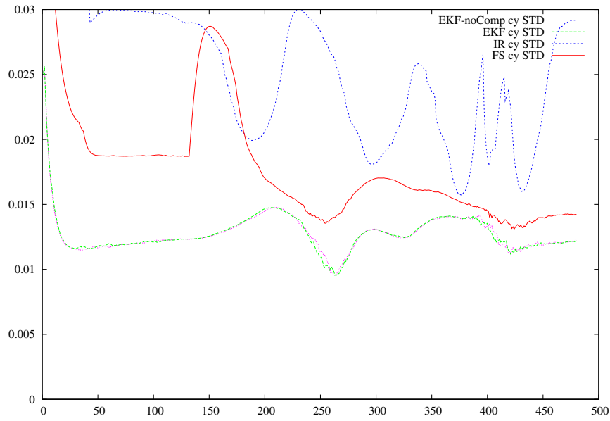
Figure 5.42: Center position standard deviation (Y coordinate).
