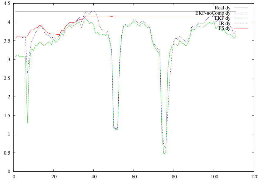
Figure 5.57: Size estimation (Y coordinate).
