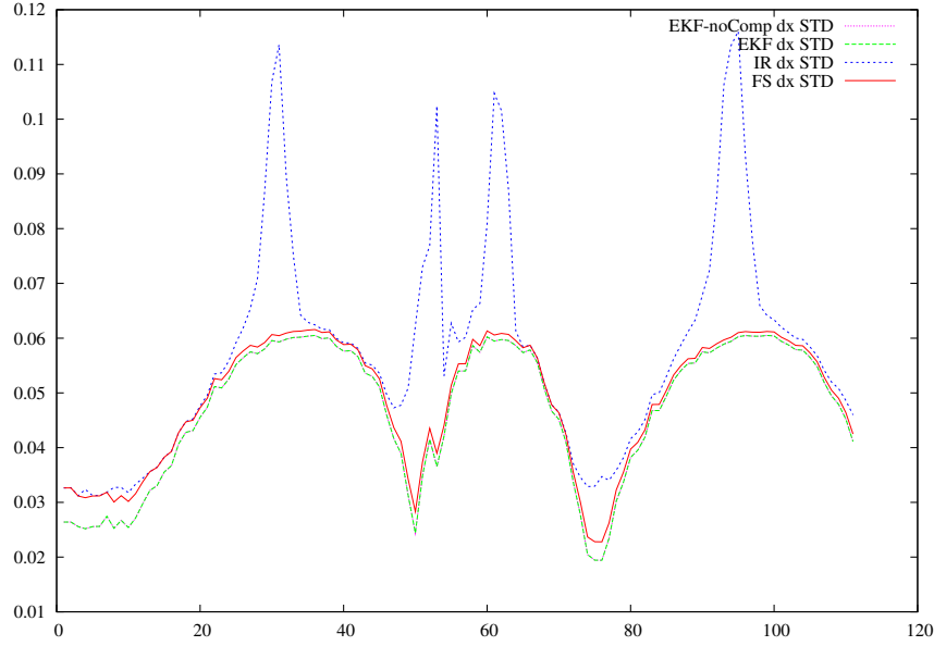
Figure 5.55: Size standard deviation (X coordinate).
