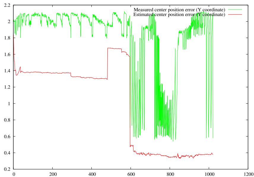
Figure 6.31: Tracked object centre's position error - Y coordinate.
