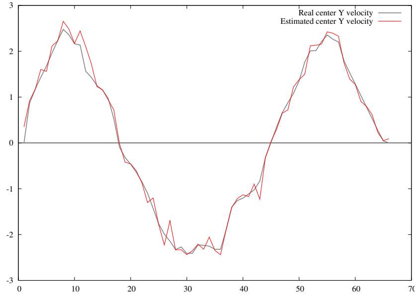
Figure 5.77: Linear velocity estimation for simulated data obtained with frequency 4Hz (Y coordinate).
