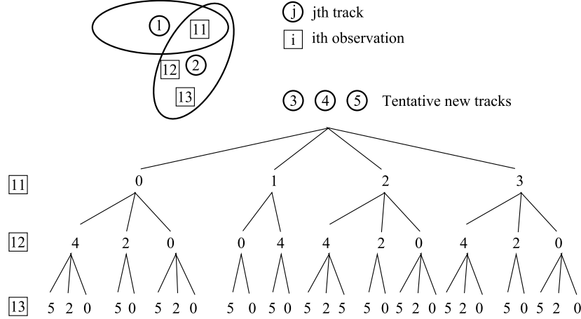
Figure 2.6: Example of hypothesis tree graph for a given configuration of targets and measurement.
