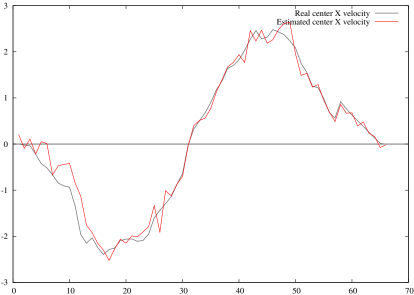
Figure 5.75: Linear velocity estimation for simulated data obtained with frequency 4Hz (X coordinate).
