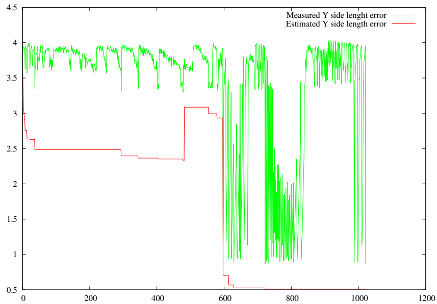
Figure 6.33: Tracked object side error - Y coordinate.
