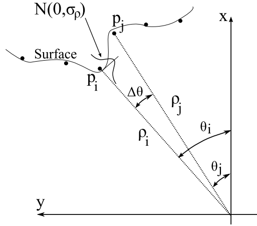
Figure 2.1: Laser scan.
