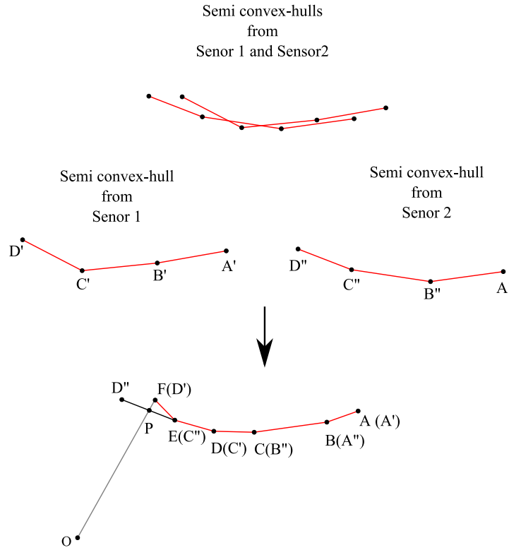
Figure 5.78: Semi convex hulls fusion.
