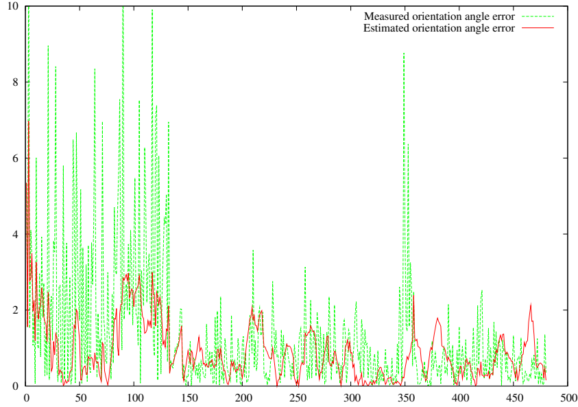
Figure 5.26: Difference between real and estimated orientation angles.
