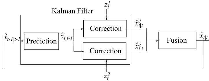
Figure 2.9: Modified track-to-track fusion schema.
