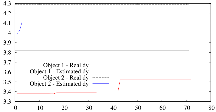
Figure 6.16: First scenario - Evolution of the vehicles' size ( Y side) using the NN method with the IR and FS based tracking.
