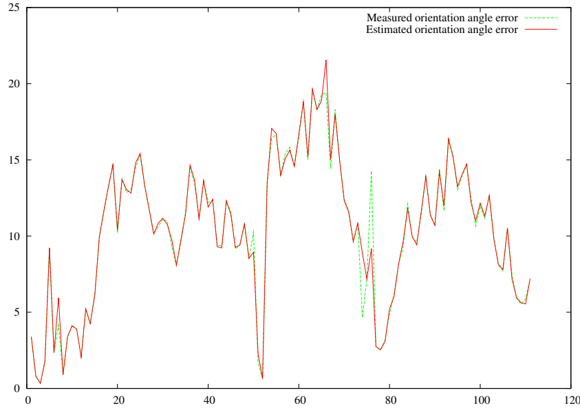
Figure 5.53: Difference between real and estimated orientation angles.
