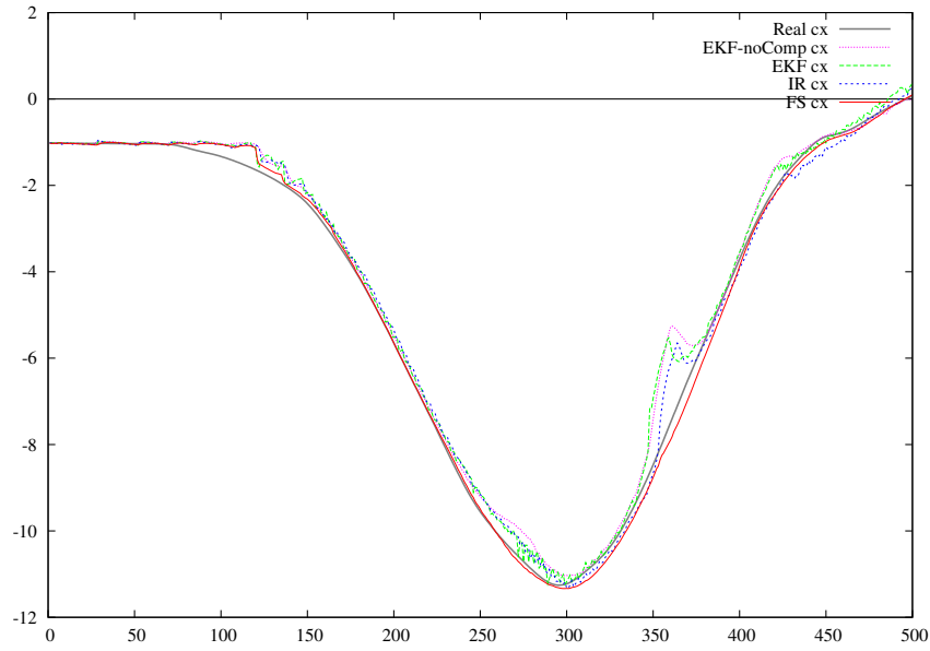
Figure 5.38: Center position estimation (X coordinate).
