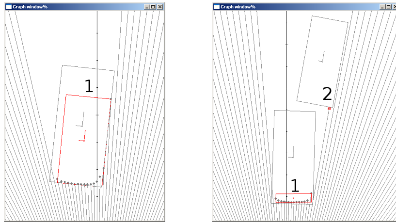
Figure 6.28: Data association results LRF-stereovision fusion based data clustering for the "vehicle turning" situation (left); and for the "vehicle occlusion" one (right).
