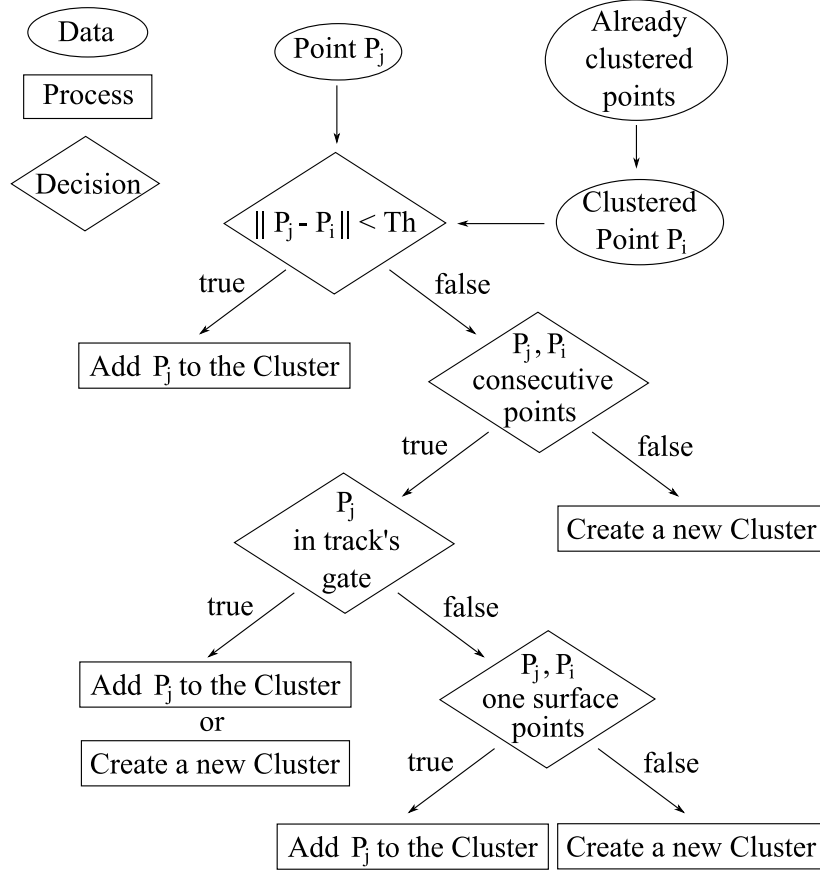
Figure 6.22: Clustering schema.
