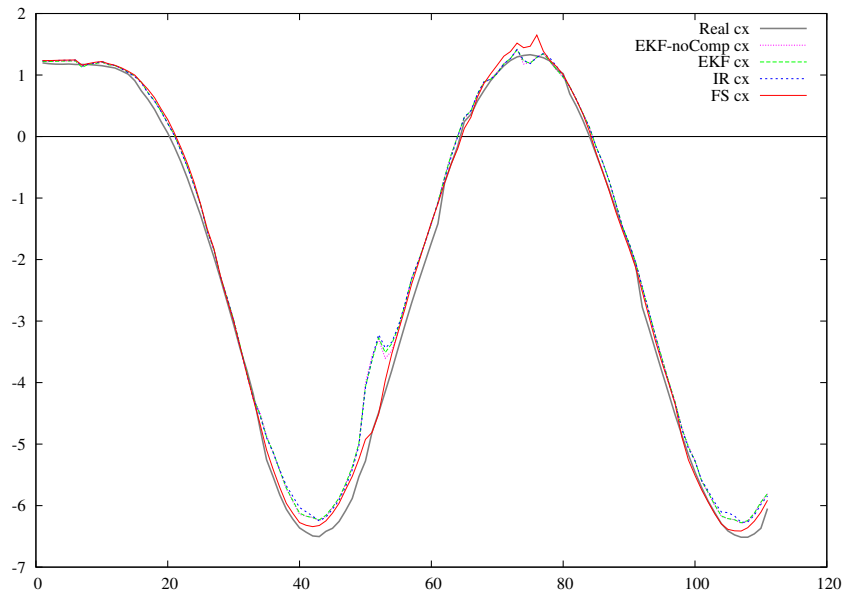
Figure 5.62: Center position estimation (X coordinate).
