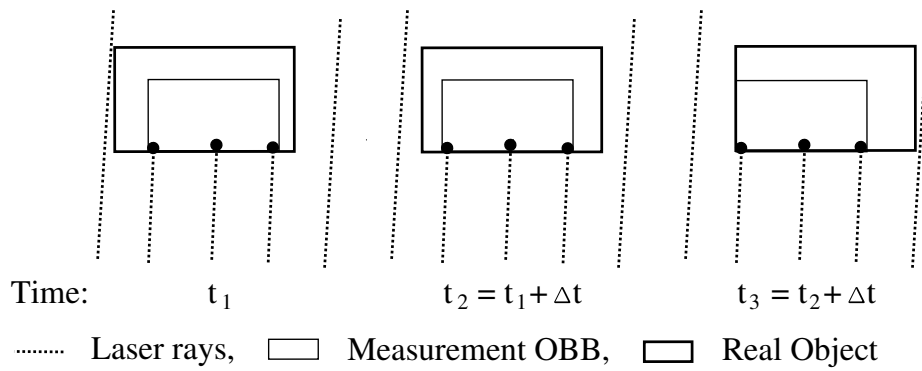
Figure 5.94: Example of the measurement OBB extraction for different object positions for greater distances (small LRF resolutions).
