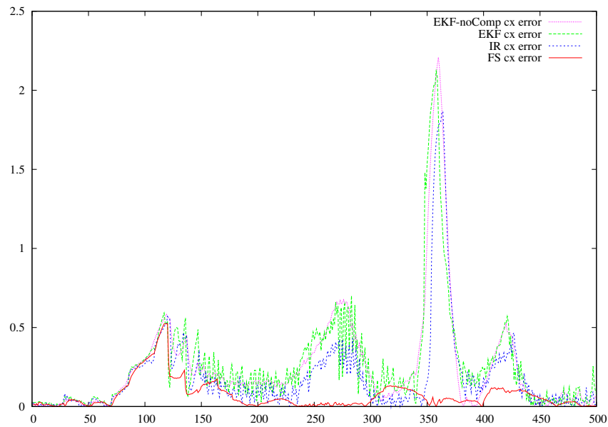
Figure 5.40: Difference between real and estimated Center positions (X coordinate).
