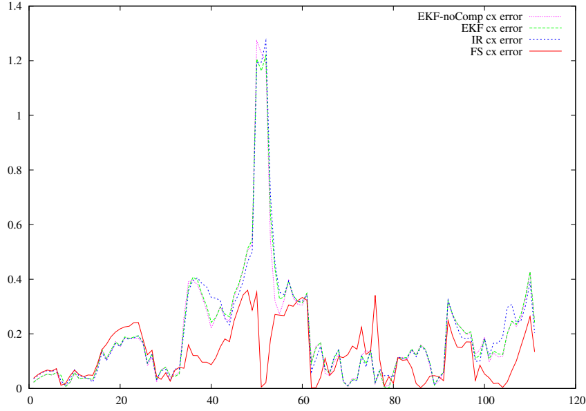
Figure 5.64: Difference between real and estimated Center positions (X coordinate).
