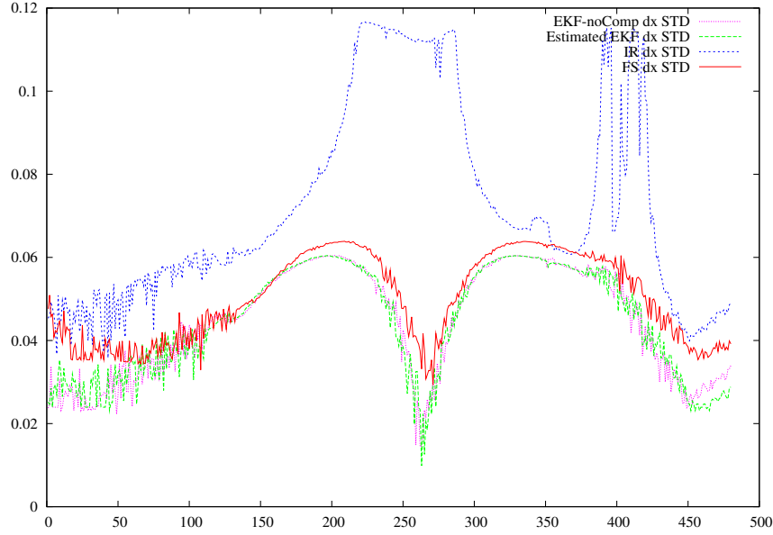
Figure 5.31: Size standard deviation (X coordinate).
