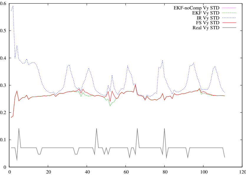
Figure 5.72: Linear velocity standard deviation (Y coordinate).
