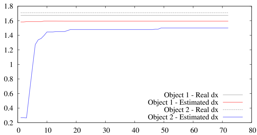
Figure 6.15: First scenario - Evolution of the vehicles' size ( X side) using the NN method with the IR and FS based tracking.
