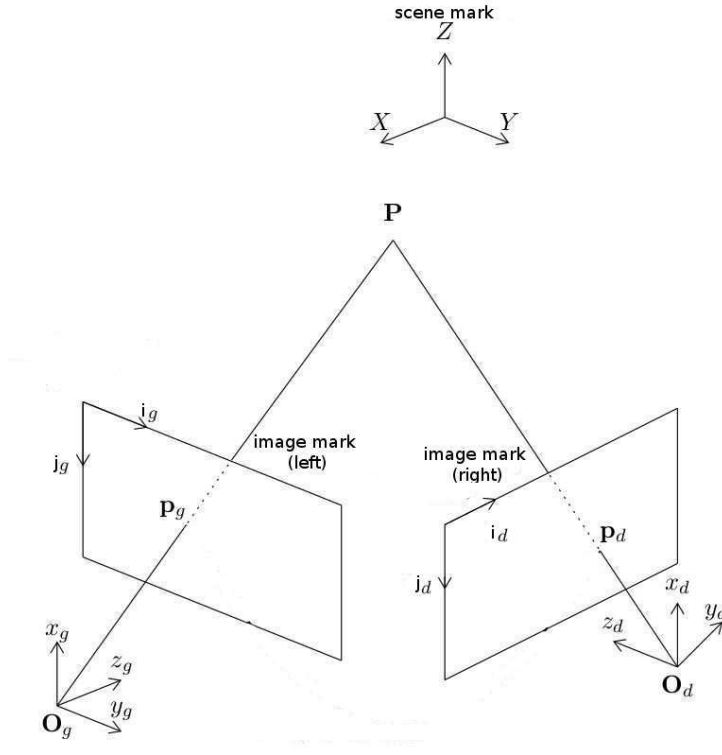
Figure 2.11: Geometric model of a binocular stereoscopic sensor
