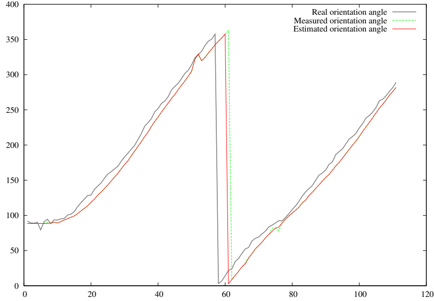
Figure 5.51: Orientation angle estimation.
