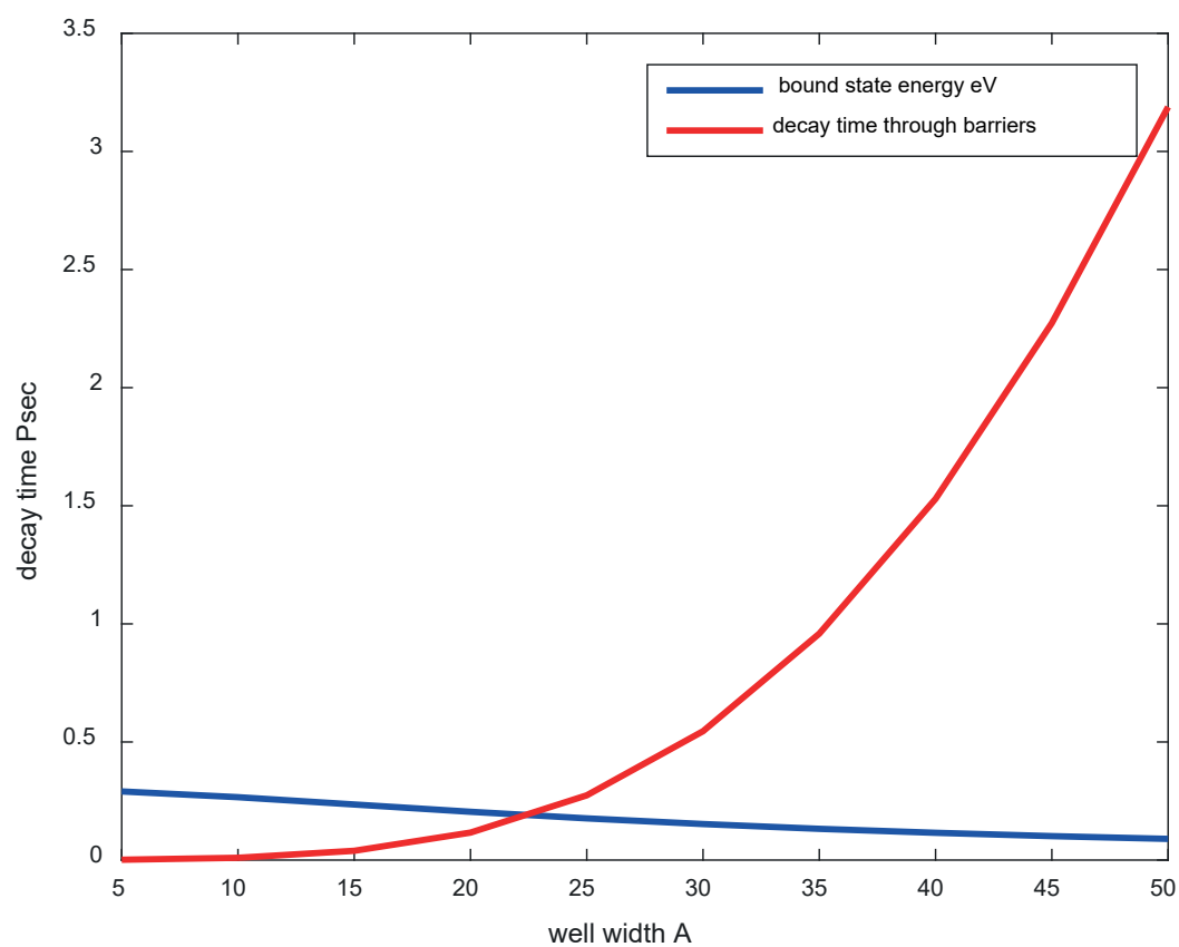
Fig. 9. The change in decay time with the width of the well
