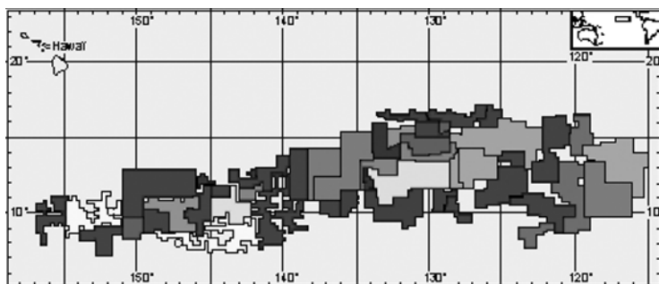
Rys. 1. Pole Clarion–Clipperton [21]
